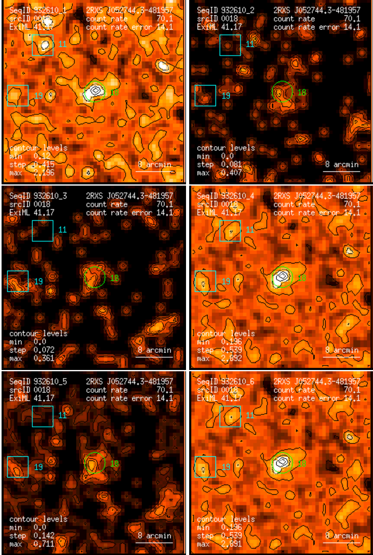
Figure 18: RASS 932610: detection 0018: band rate images, Gaussian filter: (1) PSPC channels 11 – 41, (2) 52 – 90, (3) 91 – 201, (4) 11 – 235, (5) 52 – 201, (6) 11 – 201. Broad band rates in counts/ks. Band rate contour levels in counts/ks/arcmin 2 .
