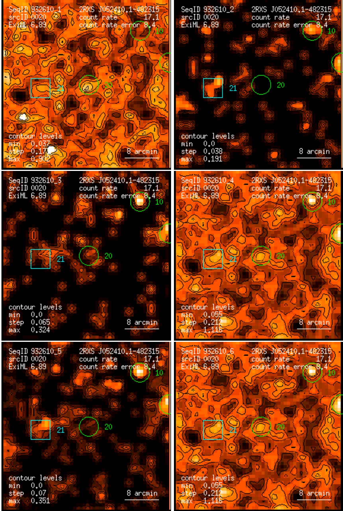
Figure 20: RASS 932610: detection 0020: band rate images, Gaussian filter: (1) PSPC channels 11 – 41, (2) 52 – 90, (3) 91 – 201, (4) 11 – 235, (5) 52 – 201, (6) 11 – 201. Broad band rates in counts/ks. Band rate contour levels in counts/ks/arcmin 2 .
