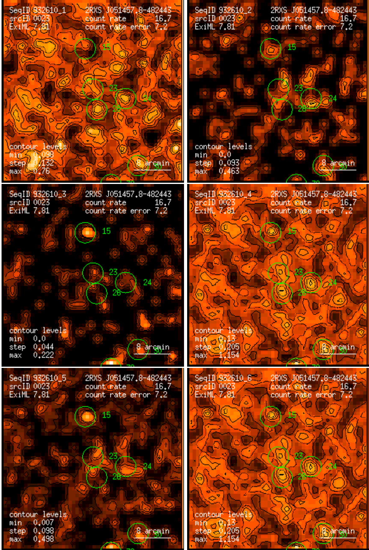
Figure 23: RASS 932610: detection 0023: band rate images, Gaussian filter: (1) PSPC channels 11 – 41, (2) 52 – 90, (3) 91 – 201, (4) 11 – 235, (5) 52 – 201, (6) 11 – 201. Broad band rates in counts/ks. Band rate contour levels in counts/ks/arcmin 2 .
