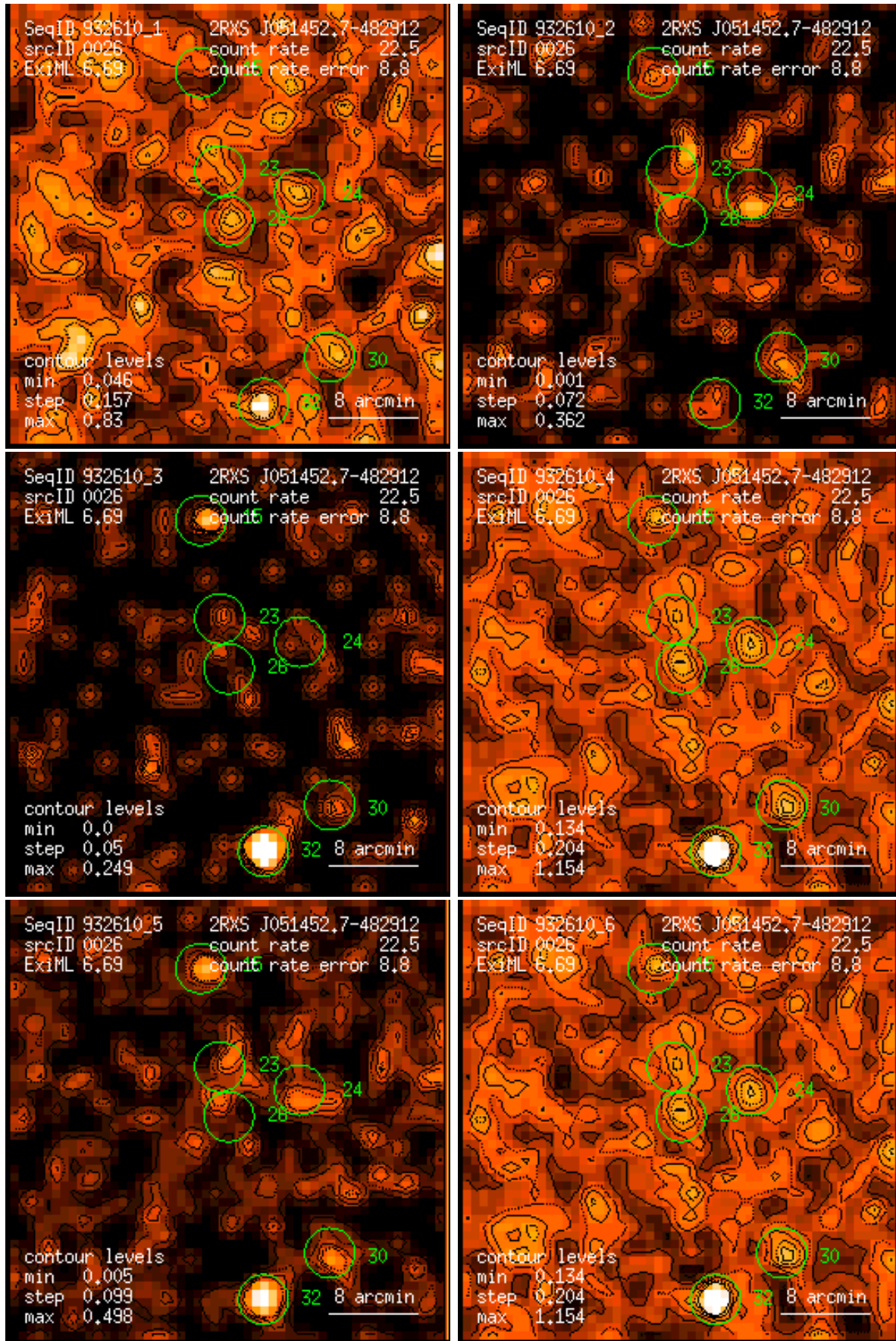
Figure 26: RASS 932610: detection 0026: band rate images, Gaussian filter: (1) PSPC channels 11 – 41, (2) 52 – 90, (3) 91 – 201, (4) 11 – 235, (5) 52 – 201, (6) 11 – 201. Broad band rates in counts/ks. Band rate contour levels in counts/ks/arcmin 2 .
