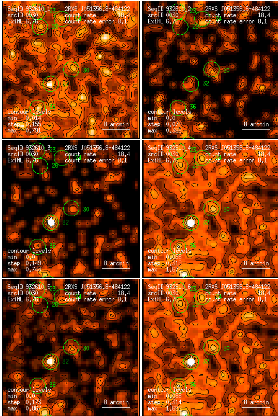
Figure 30: RASS 932610: detection 0030: band rate images, Gaussian filter: (1) PSPC channels 11 – 41, (2) 52 – 90, (3) 91 – 201, (4) 11 – 235, (5) 52 – 201, (6) 11 – 201. Broad band rates in counts/ks. Band rate contour levels in counts/ks/arcmin 2 .
