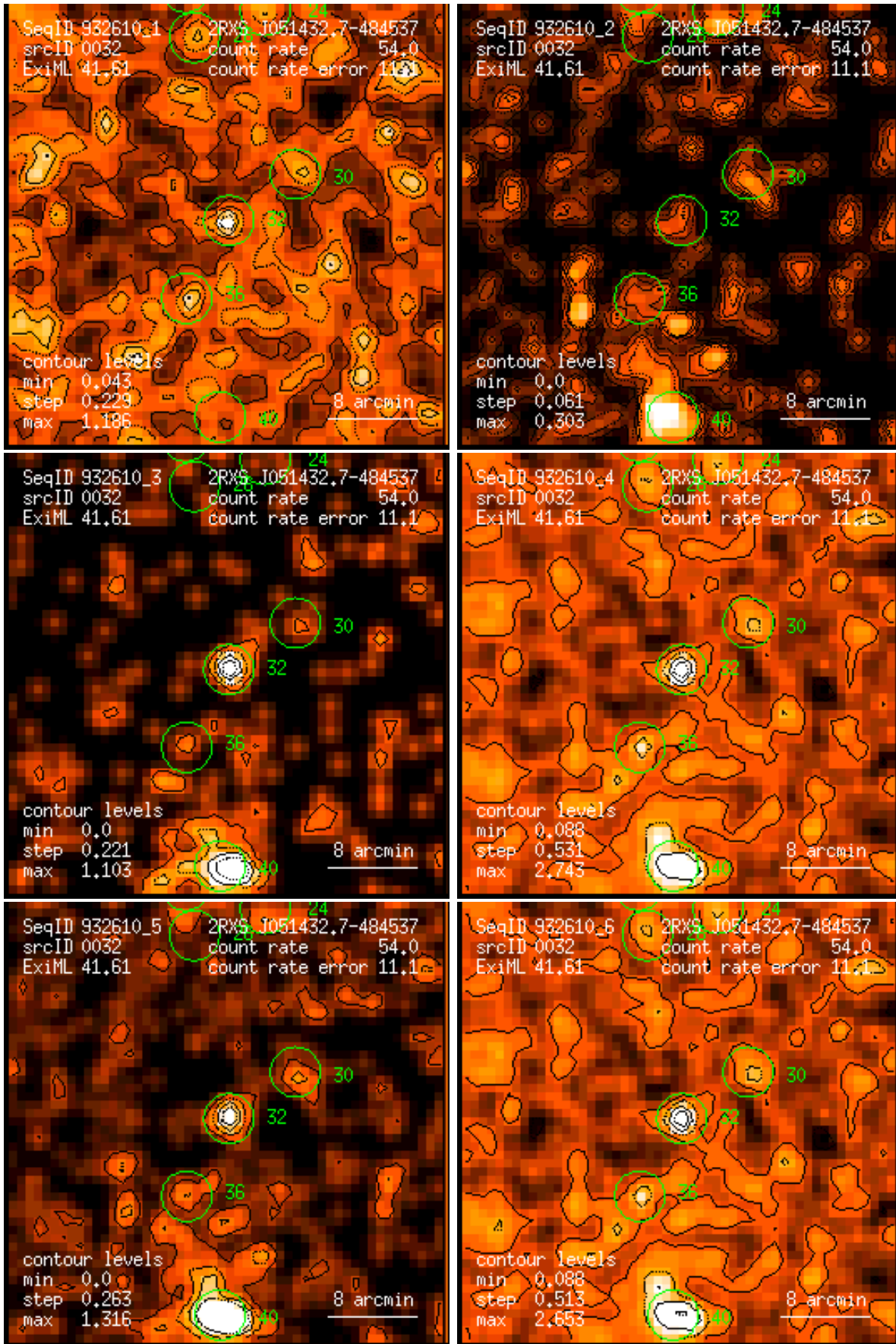
Figure 32: RASS 932610: detection 0032: band rate images, Gaussian filter: (1) PSPC channels 11 – 41, (2) 52 – 90, (3) 91 – 201, (4) 11 – 235, (5) 52 – 201, (6) 11 – 201. Broad band rates in counts/ks. Band rate contour levels in counts/ks/arcmin 2 .
