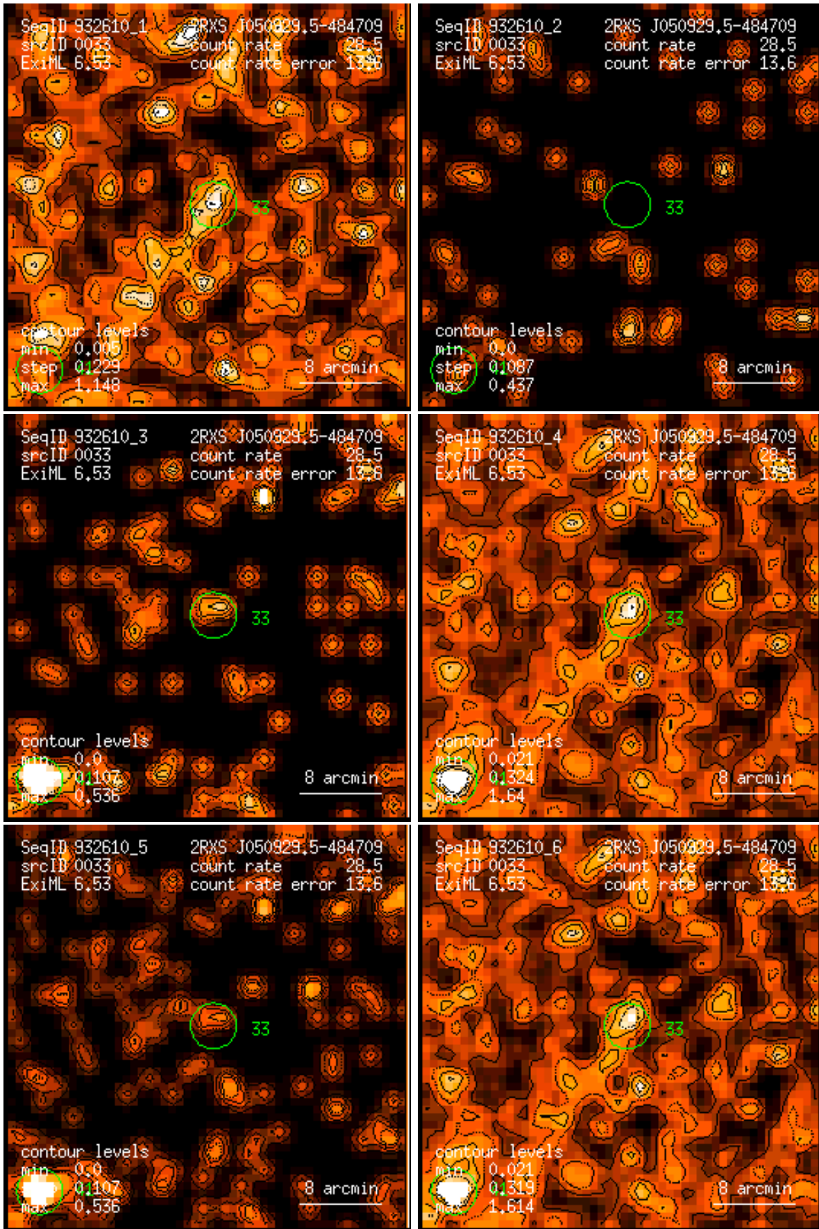
Figure 33: RASS 932610: detection 0033: band rate images, Gaussian filter: (1) PSPC channels 11 – 41, (2) 52 – 90, (3) 91 – 201, (4) 11 – 235, (5) 52 – 201, (6) 11 – 201. Broad band rates in counts/ks. Band rate contour levels in counts/ks/arcmin 2 .
