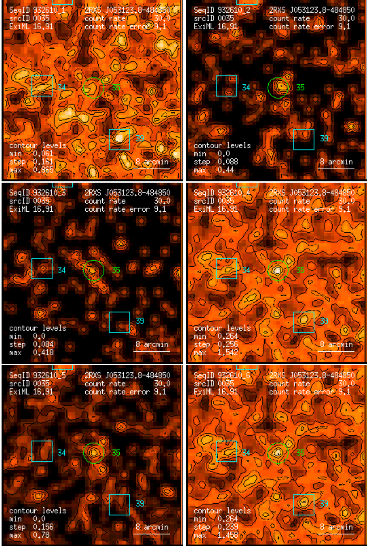
Figure 35: RASS 932610: detection 0035: band rate images, Gaussian filter: (1) PSPC channels 11 – 41, (2) 52 – 90, (3) 91 – 201, (4) 11 – 235, (5) 52 – 201, (6) 11 – 201. Broad band rates in counts/ks. Band rate contour levels in counts/ks/arcmin 2 .
