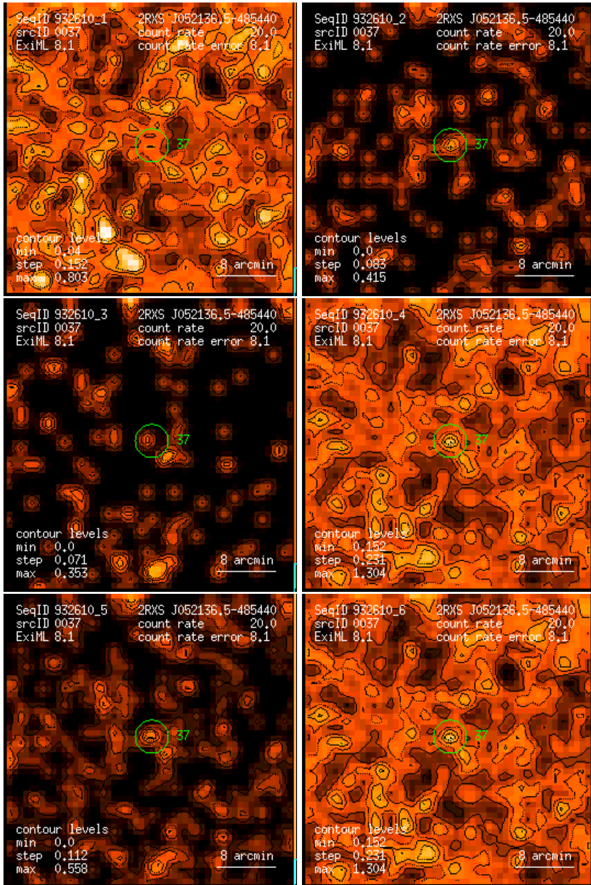
Figure 37: RASS 932610: detection 0037: band rate images, Gaussian filter: (1) PSPC channels 11 – 41, (2) 52 – 90, (3) 91 – 201, (4) 11 – 235, (5) 52 – 201, (6) 11 – 201. Broad band rates in counts/ks. Band rate contour levels in counts/ks/arcmin 2 .
