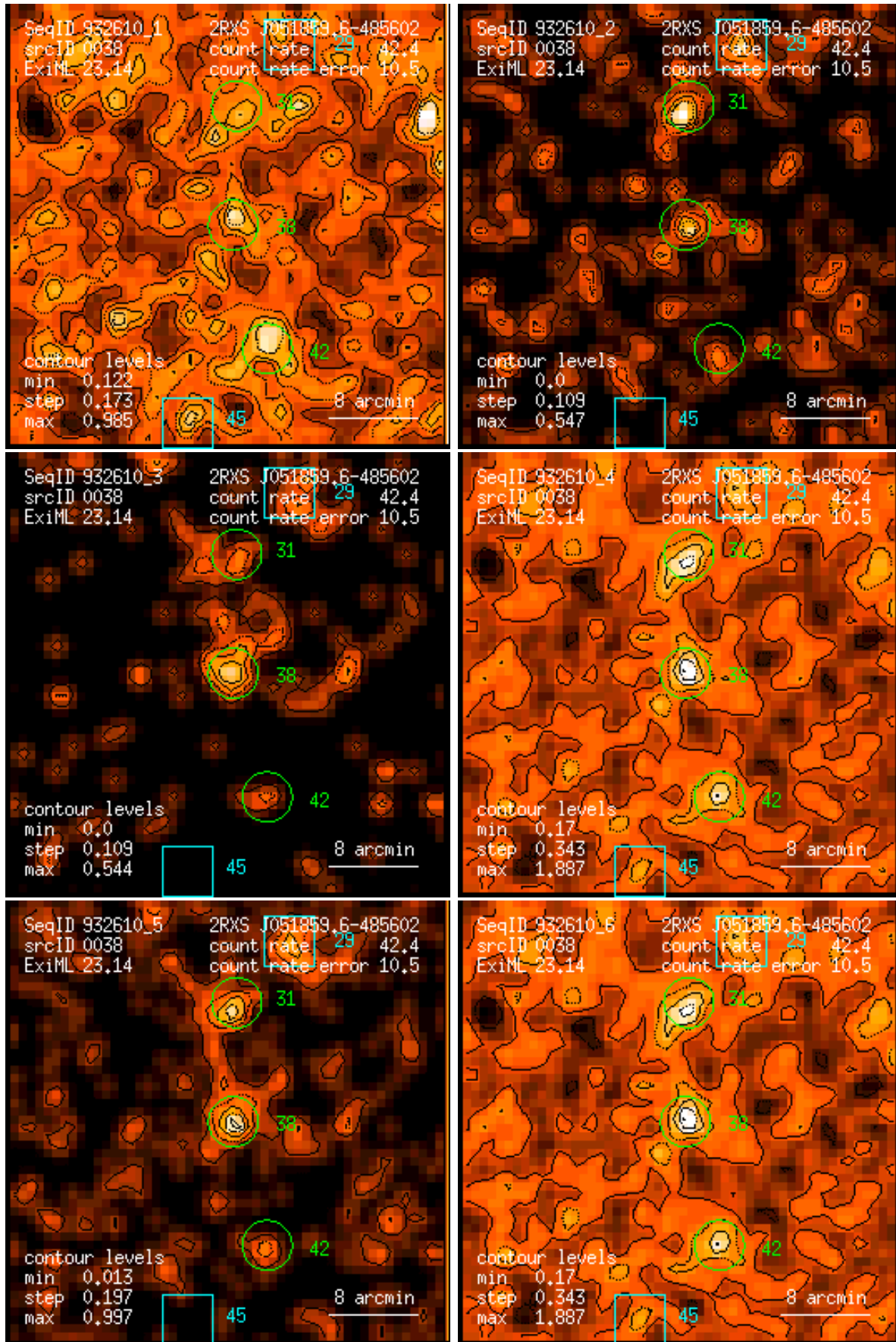
Figure 38: RASS 932610: detection 0038: band rate images, Gaussian filter: (1) PSPC channels 11 – 41, (2) 52 – 90, (3) 91 – 201, (4) 11 – 235, (5) 52 – 201, (6) 11 – 201. Broad band rates in counts/ks. Band rate contour levels in counts/ks/arcmin 2 .
