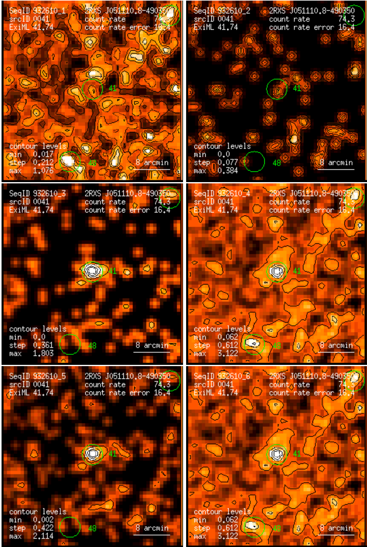
Figure 41: RASS 932610: detection 0041: band rate images, Gaussian filter: (1) PSPC channels 11 – 41, (2) 52 – 90, (3) 91 – 201, (4) 11 – 235, (5) 52 – 201, (6) 11 – 201. Broad band rates in counts/ks. Band rate contour levels in counts/ks/arcmin 2 .
