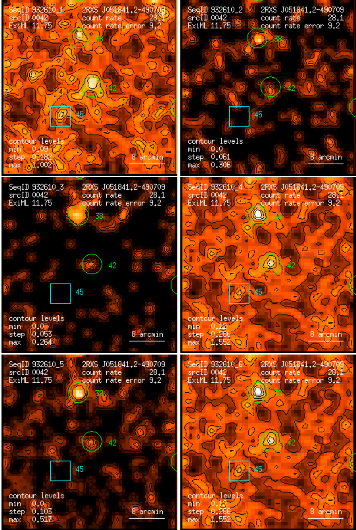
Figure 42: RASS 932610: detection 0042: band rate images, Gaussian filter: (1) PSPC channels 11 – 41, (2) 52 – 90, (3) 91 – 201, (4) 11 – 235, (5) 52 – 201, (6) 11 – 201. Broad band rates in counts/ks. Band rate contour levels in counts/ks/arcmin 2 .
