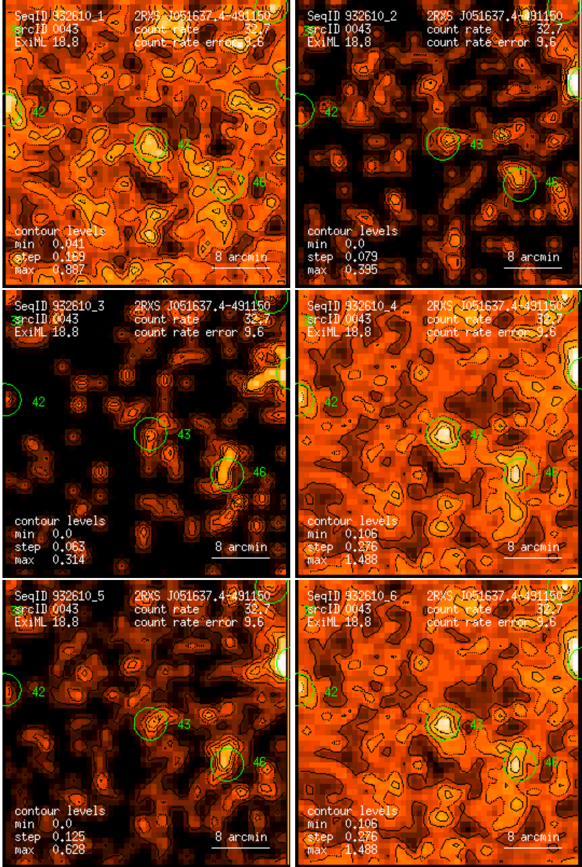
Figure 43: RASS 932610: detection 0043: band rate images, Gaussian filter: (1) PSPC channels 11 – 41, (2) 52 – 90, (3) 91 – 201, (4) 11 – 235, (5) 52 – 201, (6) 11 – 201. Broad band rates in counts/ks. Band rate contour levels in counts/ks/arcmin 2 .
