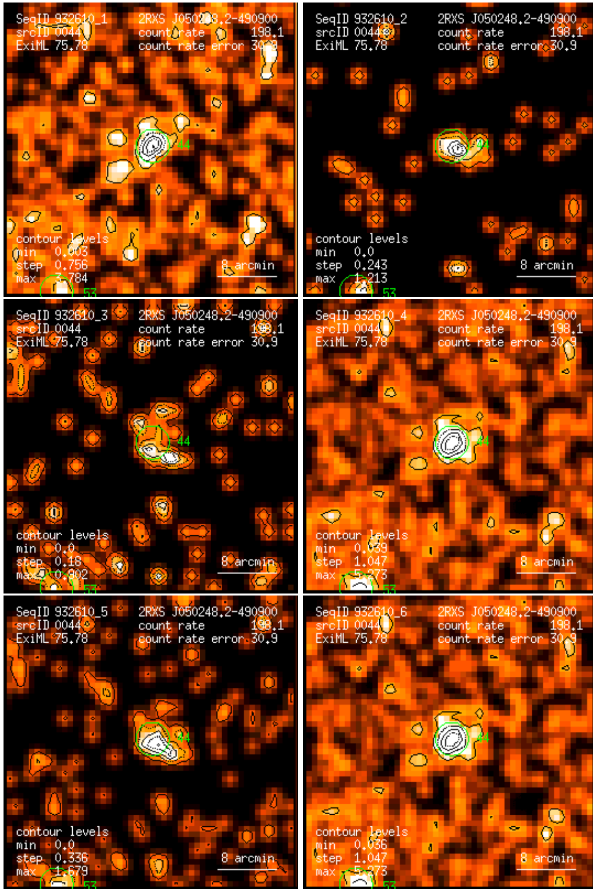
Figure 44: RASS 932610: detection 0044: band rate images, Gaussian filter: (1) PSPC channels 11 – 41, (2) 52 – 90, (3) 91 – 201, (4) 11 – 235, (5) 52 – 201, (6) 11 – 201. Broad band rates in counts/ks. Band rate contour levels in counts/ks/arcmin 2 .
