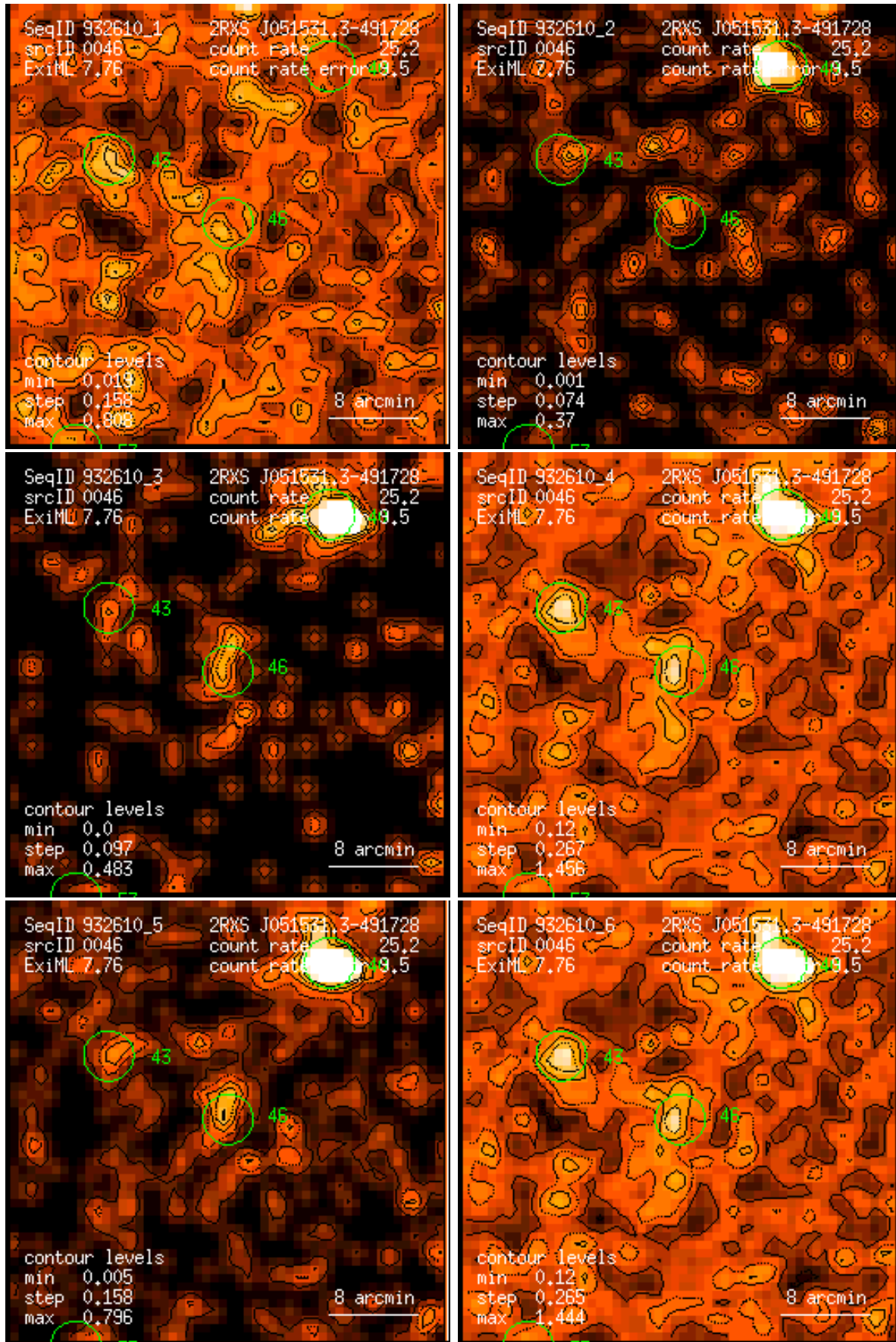
Figure 46: RASS 932610: detection 0046: band rate images, Gaussian filter: (1) PSPC channels 11 – 41, (2) 52 – 90, (3) 91 – 201, (4) 11 – 235, (5) 52 – 201, (6) 11 – 201. Broad band rates in counts/ks. Band rate contour levels in counts/ks/arcmin 2 .
