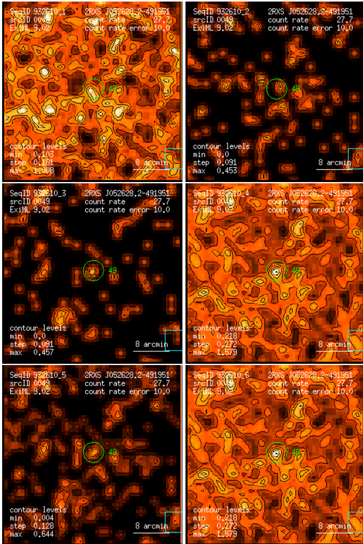
Figure 49: RASS 932610: detection 0049: band rate images, Gaussian filter: (1) PSPC channels 11 – 41, (2) 52 – 90, (3) 91 – 201, (4) 11 – 235, (5) 52 – 201, (6) 11 – 201. Broad band rates in counts/ks. Band rate contour levels in counts/ks/arcmin 2 .
