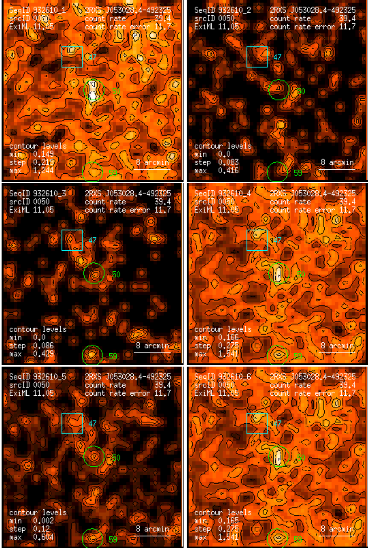
Figure 50: RASS 932610: detection 0050: band rate images, Gaussian filter: (1) PSPC channels 11 – 41, (2) 52 – 90, (3) 91 – 201, (4) 11 – 235, (5) 52 – 201, (6) 11 – 201. Broad band rates in counts/ks. Band rate contour levels in counts/ks/arcmin 2 .
