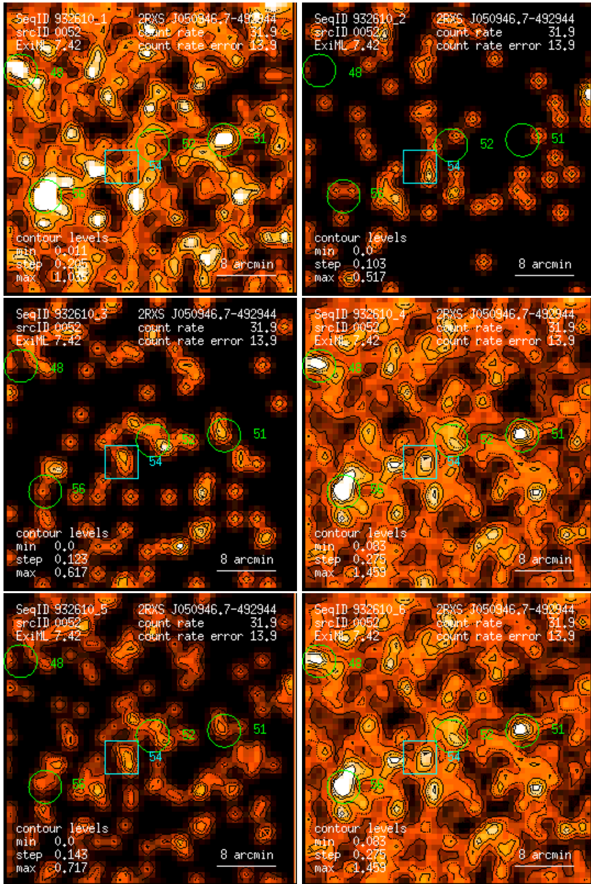
Figure 52: RASS 932610: detection 0052: band rate images, Gaussian filter: (1) PSPC channels 11 – 41, (2) 52 – 90, (3) 91 – 201, (4) 11 – 235, (5) 52 – 201, (6) 11 – 201. Broad band rates in counts/ks. Band rate contour levels in counts/ks/arcmin 2 .
