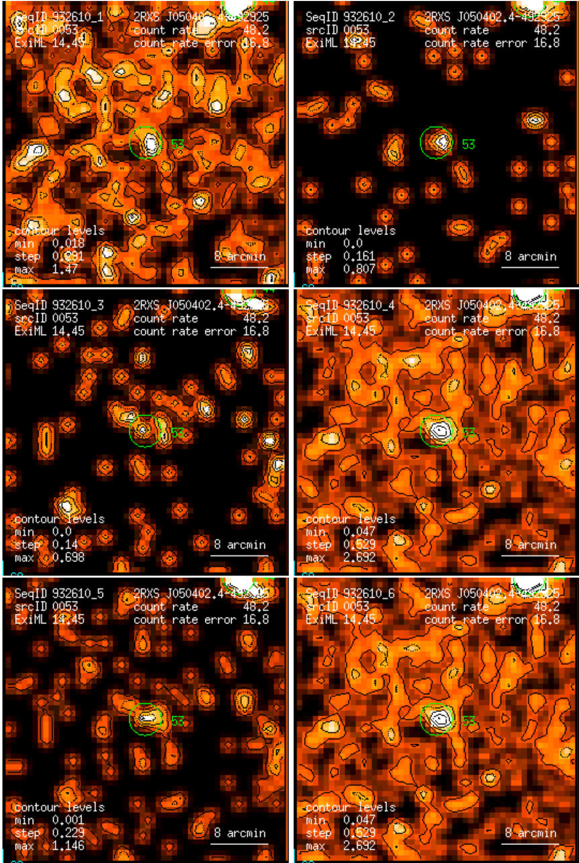
Figure 53: RASS 932610: detection 0053: band rate images, Gaussian filter: (1) PSPC channels 11 – 41, (2) 52 – 90, (3) 91 – 201, (4) 11 – 235, (5) 52 – 201, (6) 11 – 201. Broad band rates in counts/ks. Band rate contour levels in counts/ks/arcmin 2 .
