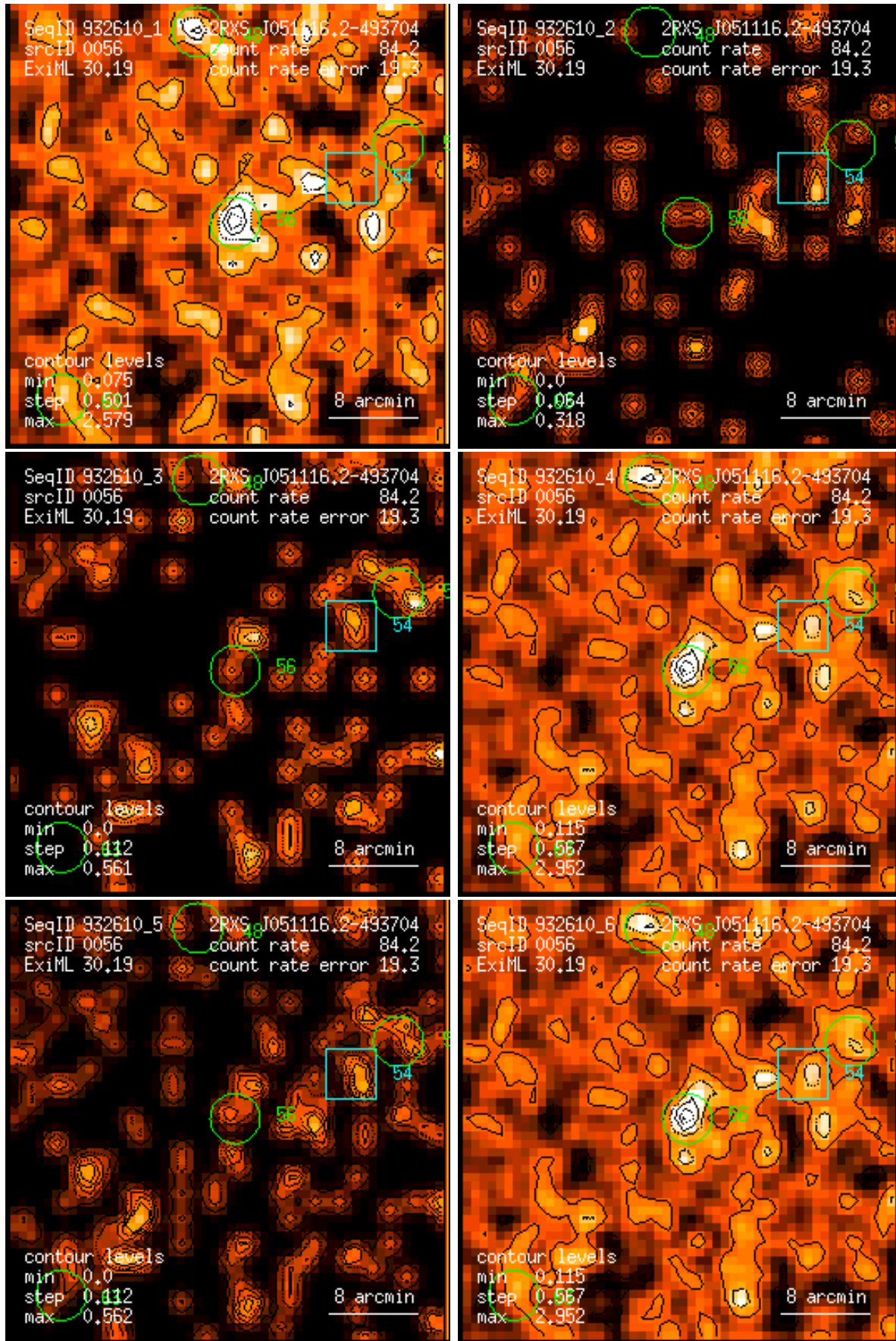
Figure 56: RASS 932610: detection 0056: band rate images, Gaussian filter: (1) PSPC channels 11 – 41, (2) 52 – 90, (3) 91 – 201, (4) 11 – 235, (5) 52 – 201, (6) 11 – 201. Broad band rates in counts/ks. Band rate contour levels in counts/ks/arcmin 2 .
