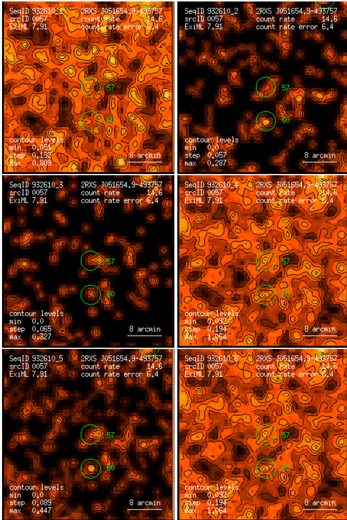
Figure 57: RASS 932610: detection 0057: band rate images, Gaussian filter: (1) PSPC channels 11 – 41, (2) 52 – 90, (3) 91 – 201, (4) 11 – 235, (5) 52 – 201, (6) 11 – 201. Broad band rates in counts/ks. Band rate contour levels in counts/ks/arcmin 2 .
