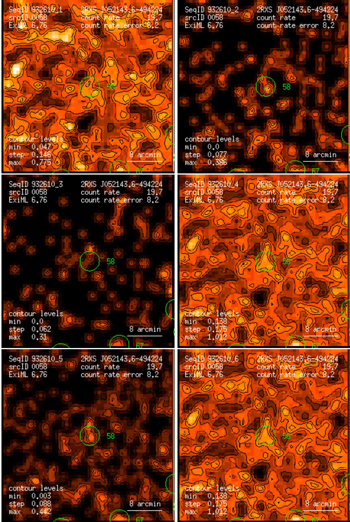
Figure 58: RASS 932610: detection 0058: band rate images, Gaussian filter: (1) PSPC channels 11 – 41, (2) 52 – 90, (3) 91 – 201, (4) 11 – 235, (5) 52 – 201, (6) 11 – 201. Broad band rates in counts/ks. Band rate contour levels in counts/ks/arcmin 2 .
