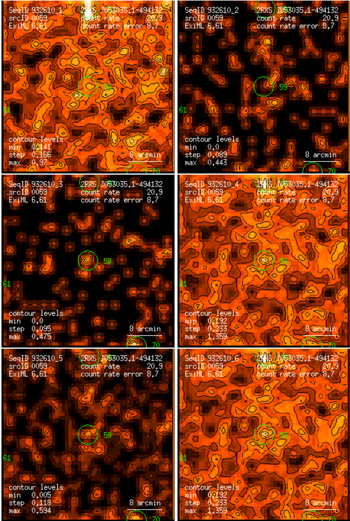
Figure 59: RASS 932610: detection 0059: band rate images, Gaussian filter: (1) PSPC channels 11 – 41, (2) 52 – 90, (3) 91 – 201, (4) 11 – 235, (5) 52 – 201, (6) 11 – 201. Broad band rates in counts/ks. Band rate contour levels in counts/ks/arcmin 2 .
