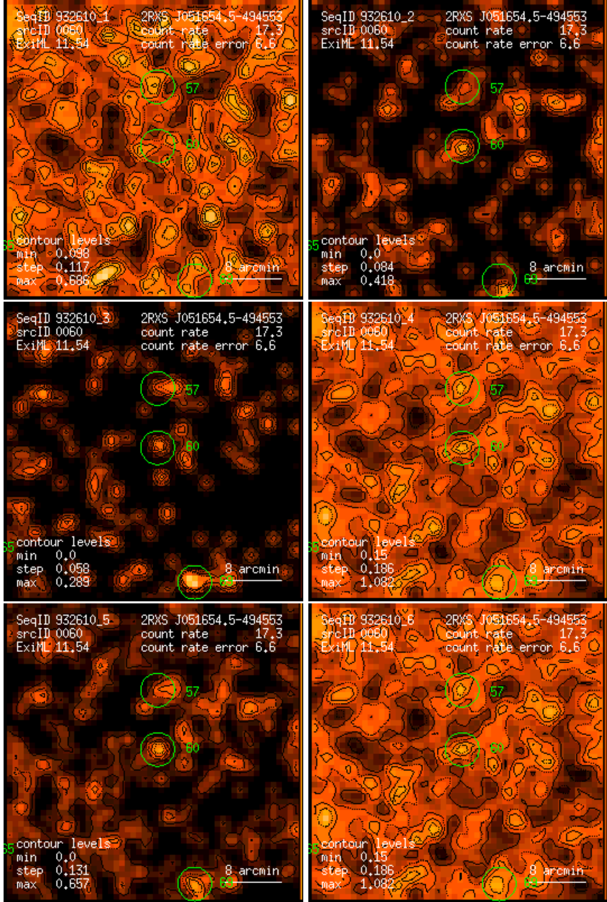
Figure 60: RASS 932610: detection 0060: band rate images, Gaussian filter: (1) PSPC channels 11 – 41, (2) 52 – 90, (3) 91 – 201, (4) 11 – 235, (5) 52 – 201, (6) 11 – 201. Broad band rates in counts/ks. Band rate contour levels in counts/ks/arcmin 2 .
