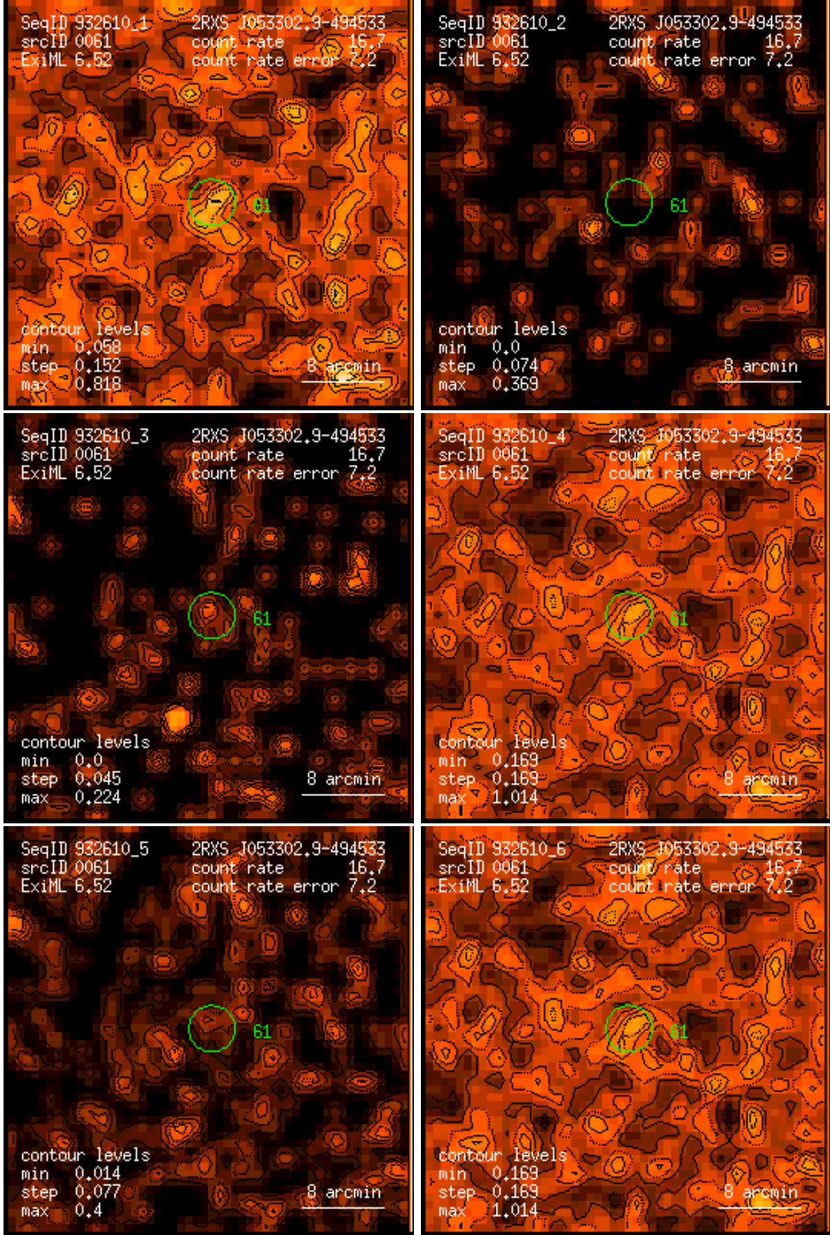
Figure 61: RASS 932610: detection 0061: band rate images, Gaussian filter: (1) PSPC channels 11 – 41, (2) 52 – 90, (3) 91 – 201, (4) 11 – 235, (5) 52 – 201, (6) 11 – 201. Broad band rates in counts/ks. Band rate contour levels in counts/ks/arcmin 2 .
