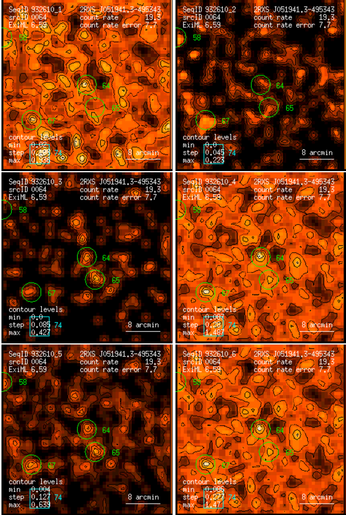
Figure 64: RASS 932610: detection 0064: band rate images, Gaussian filter: (1) PSPC channels 11 – 41, (2) 52 – 90, (3) 91 – 201, (4) 11 – 235, (5) 52 – 201, (6) 11 – 201. Broad band rates in counts/ks. Band rate contour levels in counts/ks/arcmin 2 .
