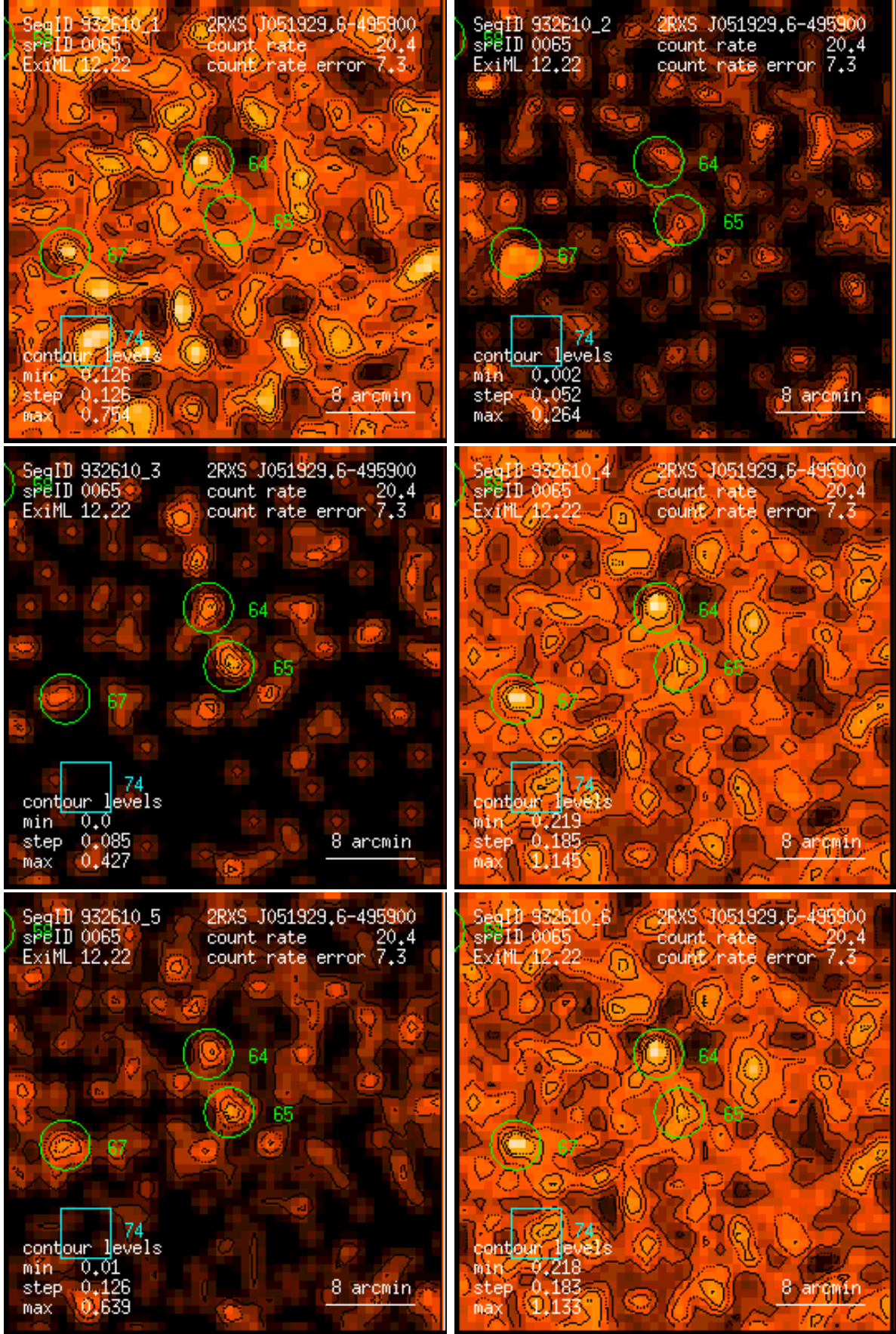
Figure 65: RASS 932610: detection 0065: band rate images, Gaussian filter: (1) PSPC channels 11 – 41, (2) 52 – 90, (3) 91 – 201, (4) 11 – 235, (5) 52 – 201, (6) 11 – 201. Broad band rates in counts/ks. Band rate contour levels in counts/ks/arcmin 2 .
