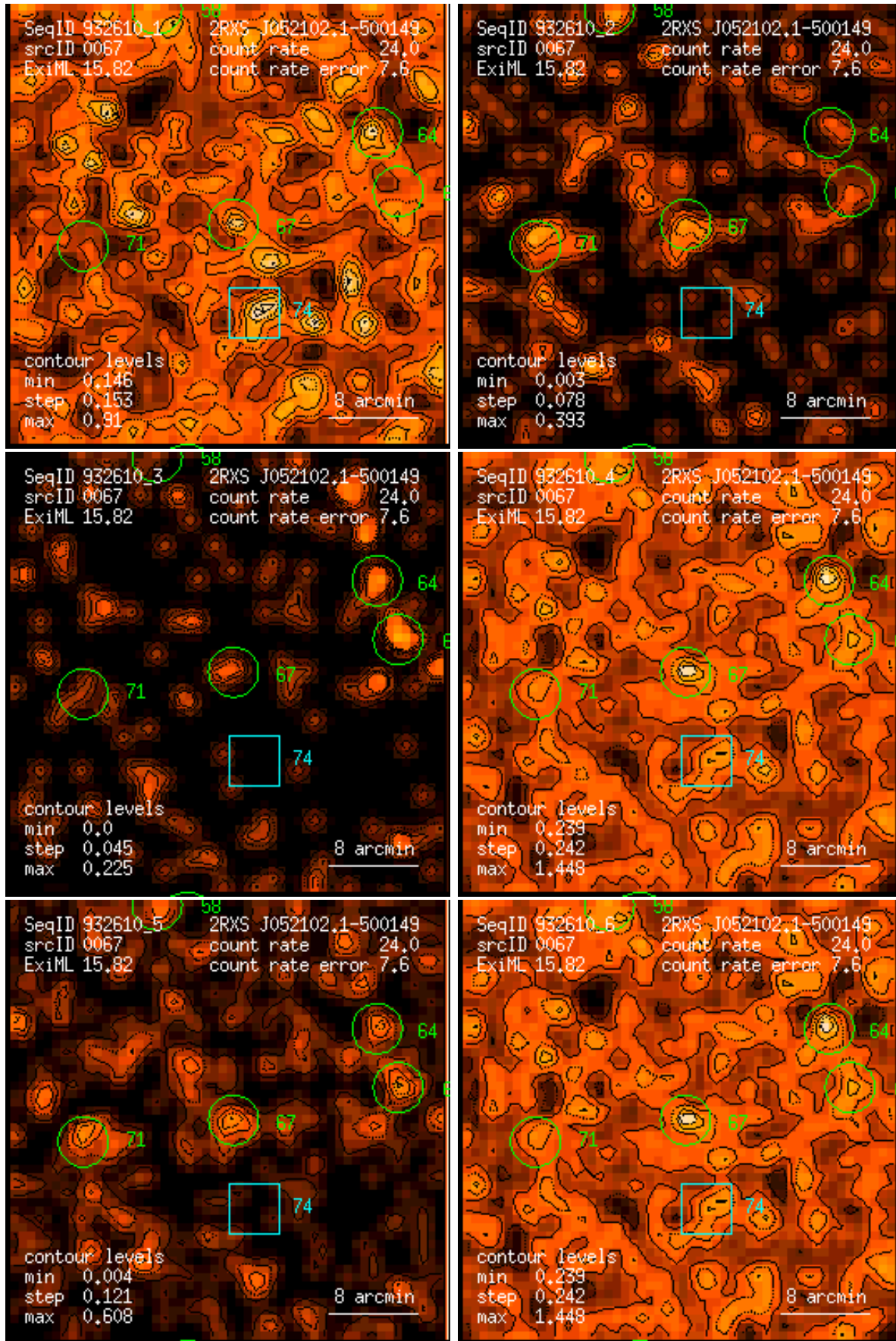
Figure 67: RASS 932610: detection 0067: band rate images, Gaussian filter: (1) PSPC channels 11 – 41, (2) 52 – 90, (3) 91 – 201, (4) 11 – 235, (5) 52 – 201, (6) 11 – 201. Broad band rates in counts/ks. Band rate contour levels in counts/ks/arcmin 2 .
