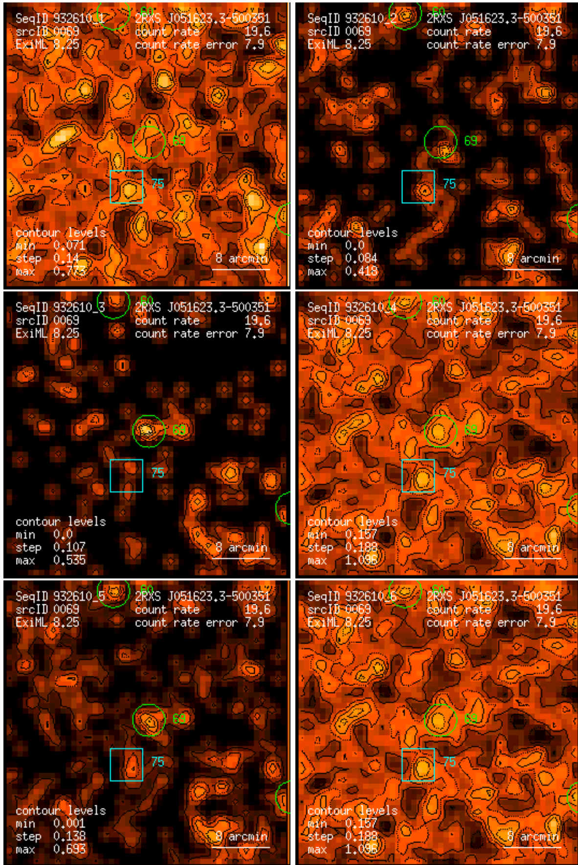
Figure 69: RASS 932610: detection 0069: band rate images, Gaussian filter: (1) PSPC channels 11 – 41, (2) 52 – 90, (3) 91 – 201, (4) 11 – 235, (5) 52 – 201, (6) 11 – 201. Broad band rates in counts/ks. Band rate contour levels in counts/ks/arcmin 2 .
