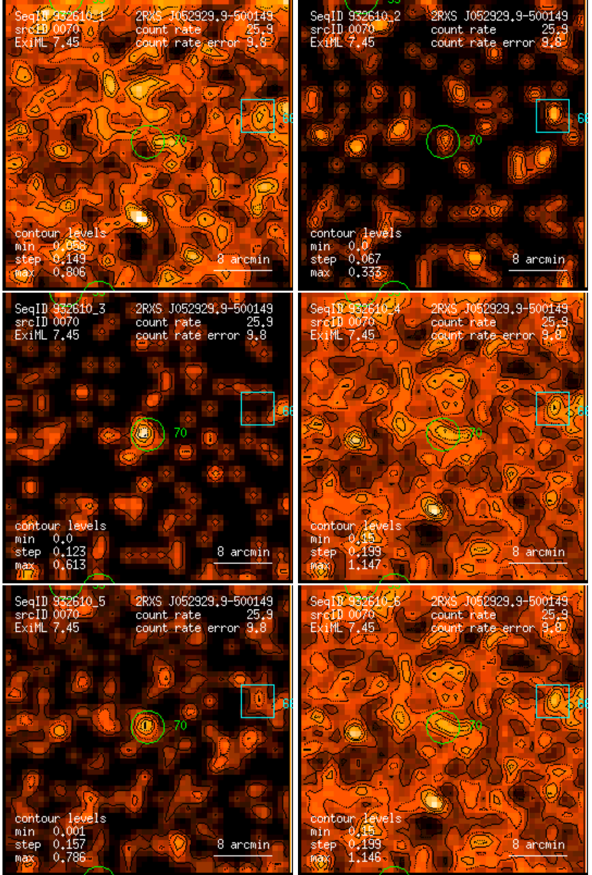
Figure 70: RASS 932610: detection 0070: band rate images, Gaussian filter: (1) PSPC channels 11 – 41, (2) 52 – 90, (3) 91 – 201, (4) 11 – 235, (5) 52 – 201, (6) 11 – 201. Broad band rates in counts/ks. Band rate contour levels in counts/ks/arcmin 2 .
