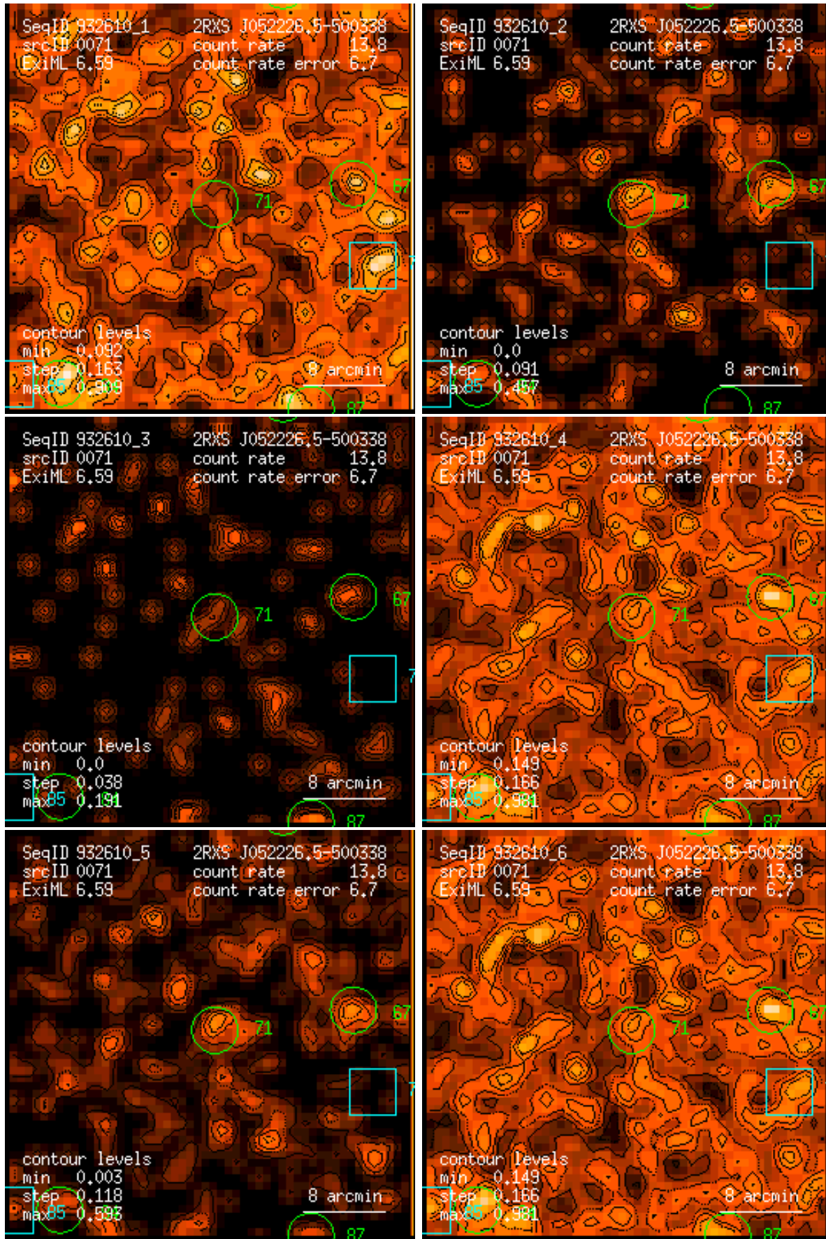
Figure 71: RASS 932610: detection 0071: band rate images, Gaussian filter: (1) PSPC channels 11 – 41, (2) 52 – 90, (3) 91 – 201, (4) 11 – 235, (5) 52 – 201, (6) 11 – 201. Broad band rates in counts/ks. Band rate contour levels in counts/ks/arcmin 2 .
