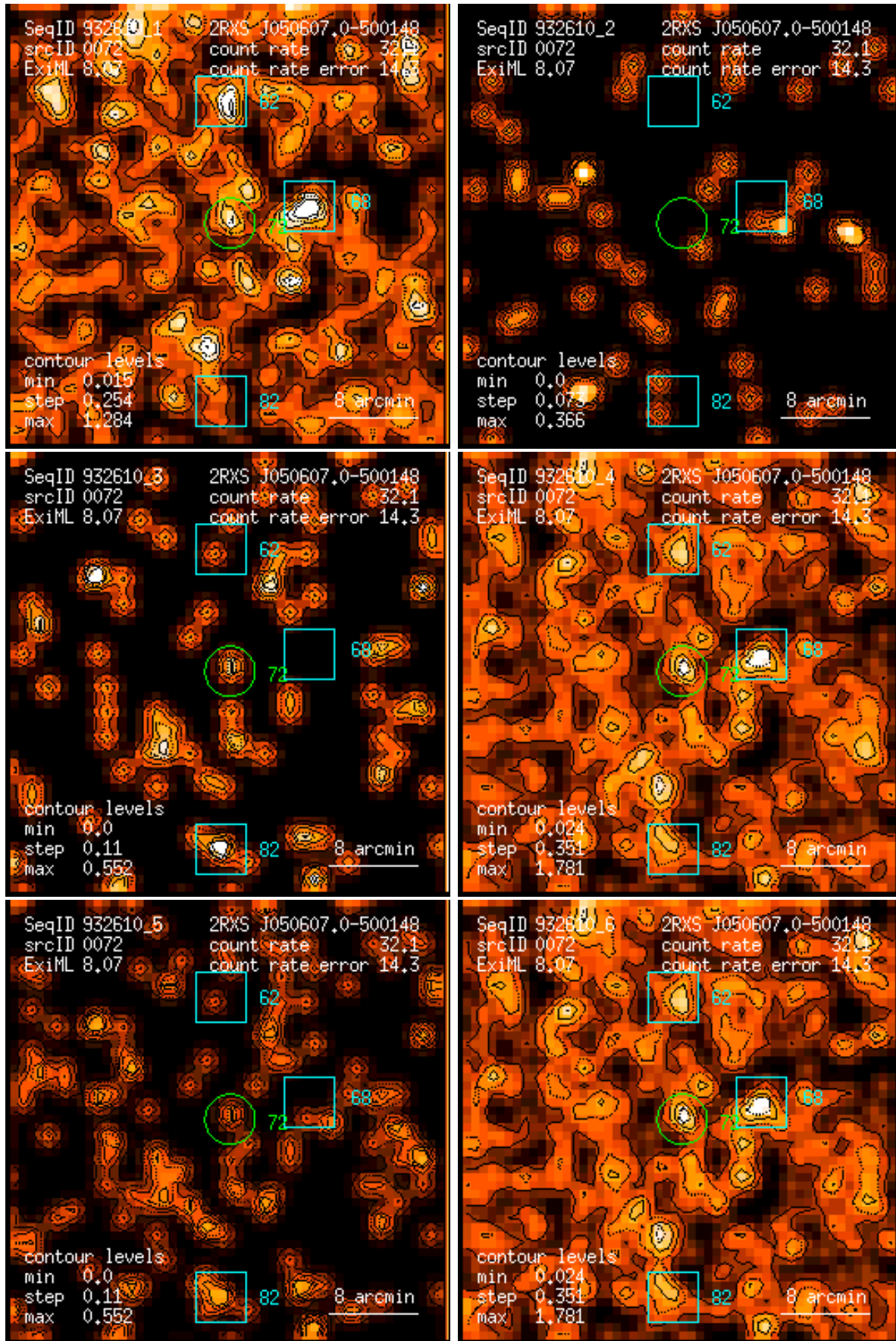
Figure 72: RASS 932610: detection 0072: band rate images, Gaussian filter: (1) PSPC channels 11 – 41, (2) 52 – 90, (3) 91 – 201, (4) 11 – 235, (5) 52 – 201, (6) 11 – 201. Broad band rates in counts/ks. Band rate contour levels in counts/ks/arcmin 2 .
