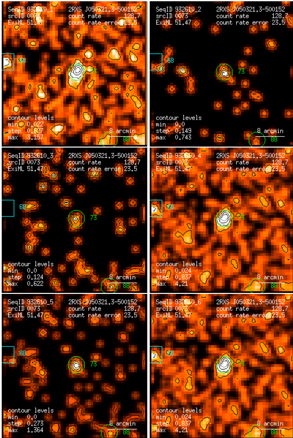
Figure 73: RASS 932610: detection 0073: band rate images, Gaussian filter: (1) PSPC channels 11 – 41, (2) 52 – 90, (3) 91 – 201, (4) 11 – 235, (5) 52 – 201, (6) 11 – 201. Broad band rates in counts/ks. Band rate contour levels in counts/ks/arcmin 2 .
