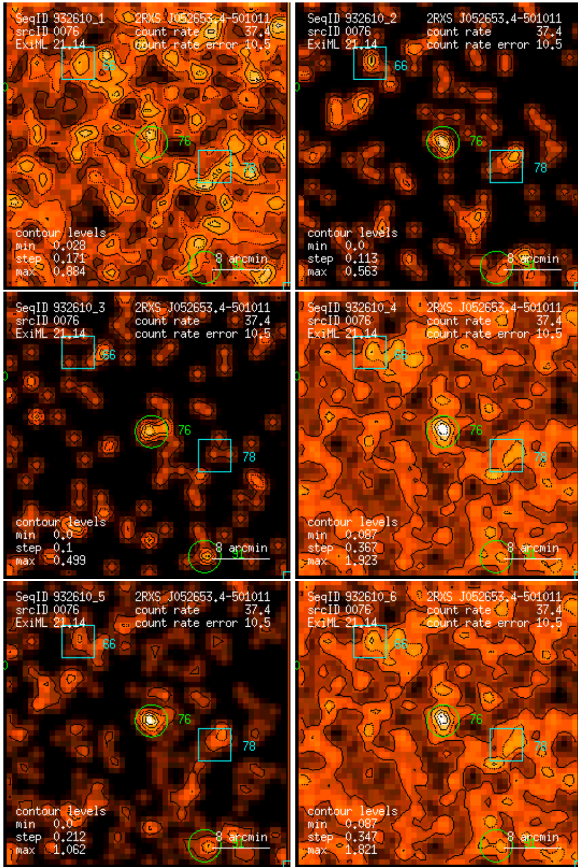
Figure 76: RASS 932610: detection 0076: band rate images, Gaussian filter: (1) PSPC channels 11 – 41, (2) 52 – 90, (3) 91 – 201, (4) 11 – 235, (5) 52 – 201, (6) 11 – 201. Broad band rates in counts/ks. Band rate contour levels in counts/ks/arcmin 2 .
