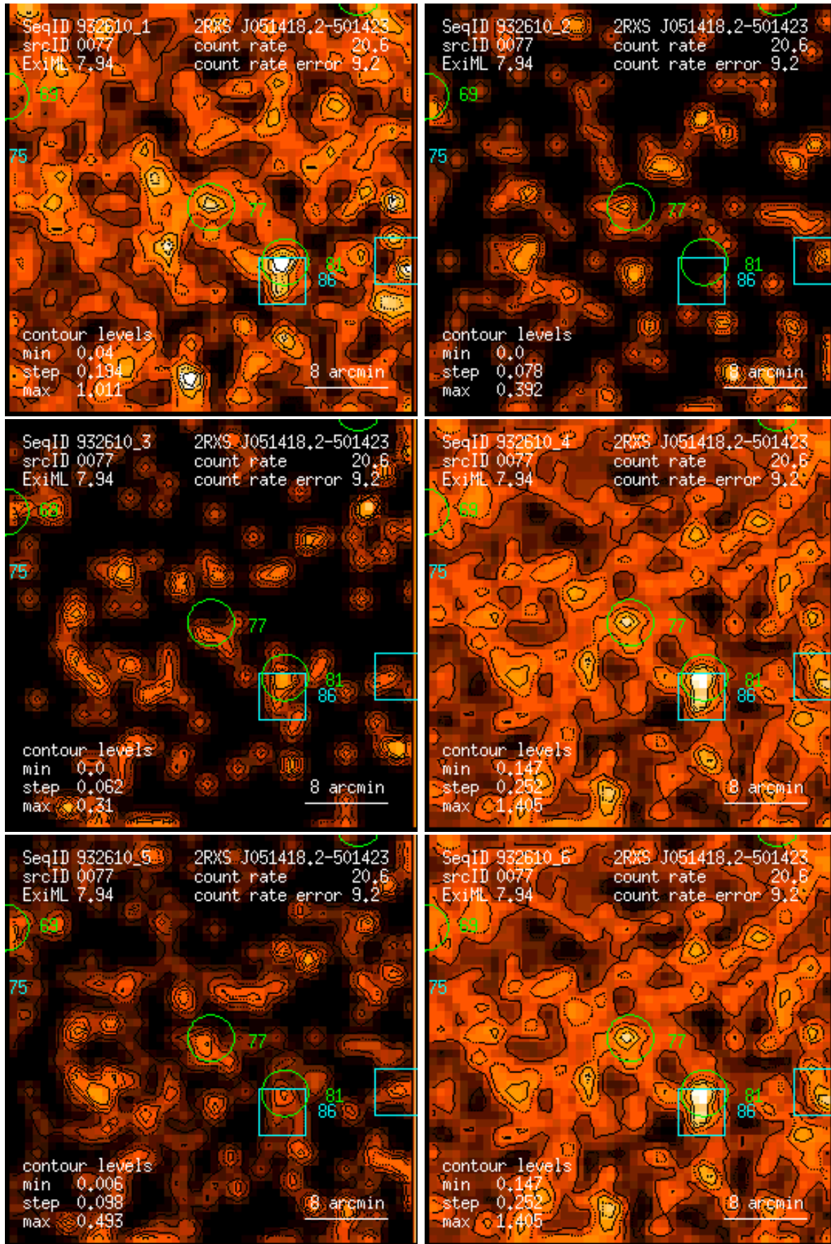
Figure 77: RASS 932610: detection 0077: band rate images, Gaussian filter: (1) PSPC channels 11 – 41, (2) 52 – 90, (3) 91 – 201, (4) 11 – 235, (5) 52 – 201, (6) 11 – 201. Broad band rates in counts/ks. Band rate contour levels in counts/ks/arcmin 2 .
