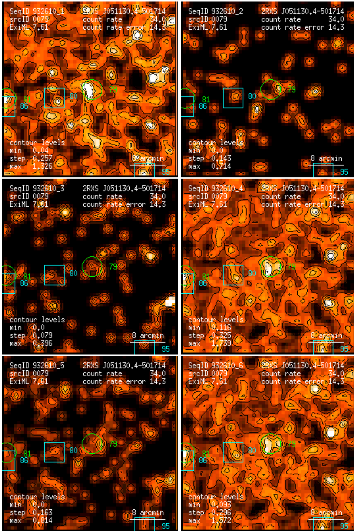
Figure 79: RASS 932610: detection 0079: band rate images, Gaussian filter: (1) PSPC channels 11 – 41, (2) 52 – 90, (3) 91 – 201, (4) 11 – 235, (5) 52 – 201, (6) 11 – 201. Broad band rates in counts/ks. Band rate contour levels in counts/ks/arcmin 2 .
