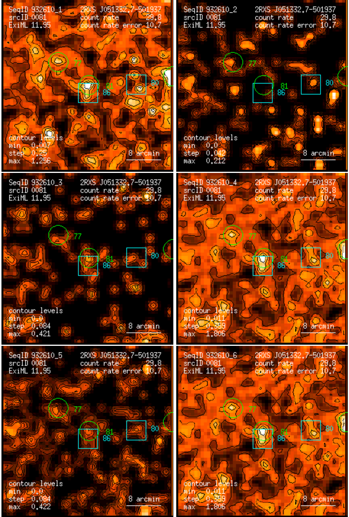
Figure 81: RASS 932610: detection 0081: band rate images, Gaussian filter: (1) PSPC channels 11 – 41, (2) 52 – 90, (3) 91 – 201, (4) 11 – 235, (5) 52 – 201, (6) 11 – 201. Broad band rates in counts/ks. Band rate contour levels in counts/ks/arcmin 2 .
