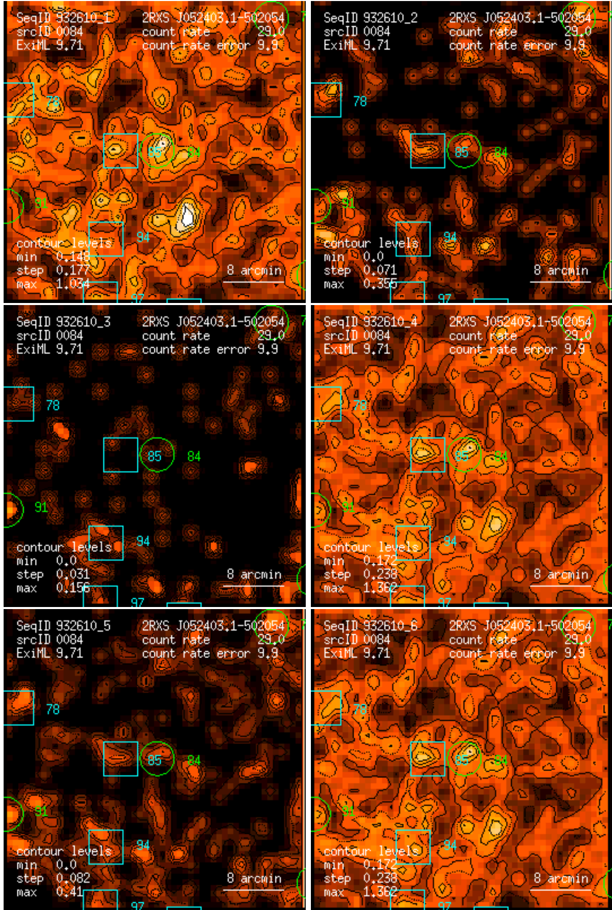
Figure 84: RASS 932610: detection 0084: band rate images, Gaussian filter: (1) PSPC channels 11 – 41, (2) 52 – 90, (3) 91 – 201, (4) 11 – 235, (5) 52 – 201, (6) 11 – 201. Broad band rates in counts/ks. Band rate contour levels in counts/ks/arcmin 2 .
