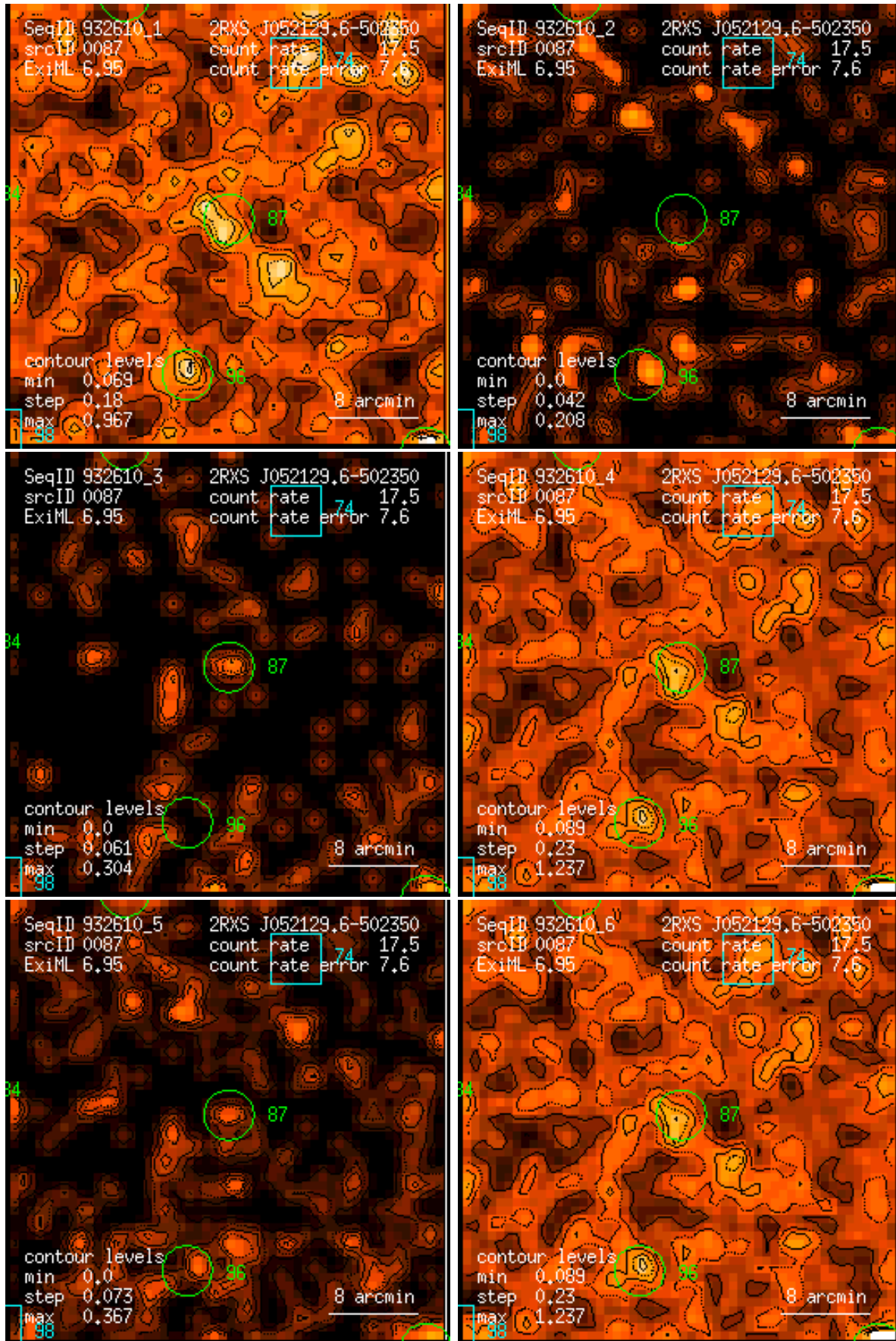
Figure 87: RASS 932610: detection 0087: band rate images, Gaussian filter: (1) PSPC channels 11 – 41, (2) 52 – 90, (3) 91 – 201, (4) 11 – 235, (5) 52 – 201, (6) 11 – 201. Broad band rates in counts/ks. Band rate contour levels in counts/ks/arcmin 2 .
