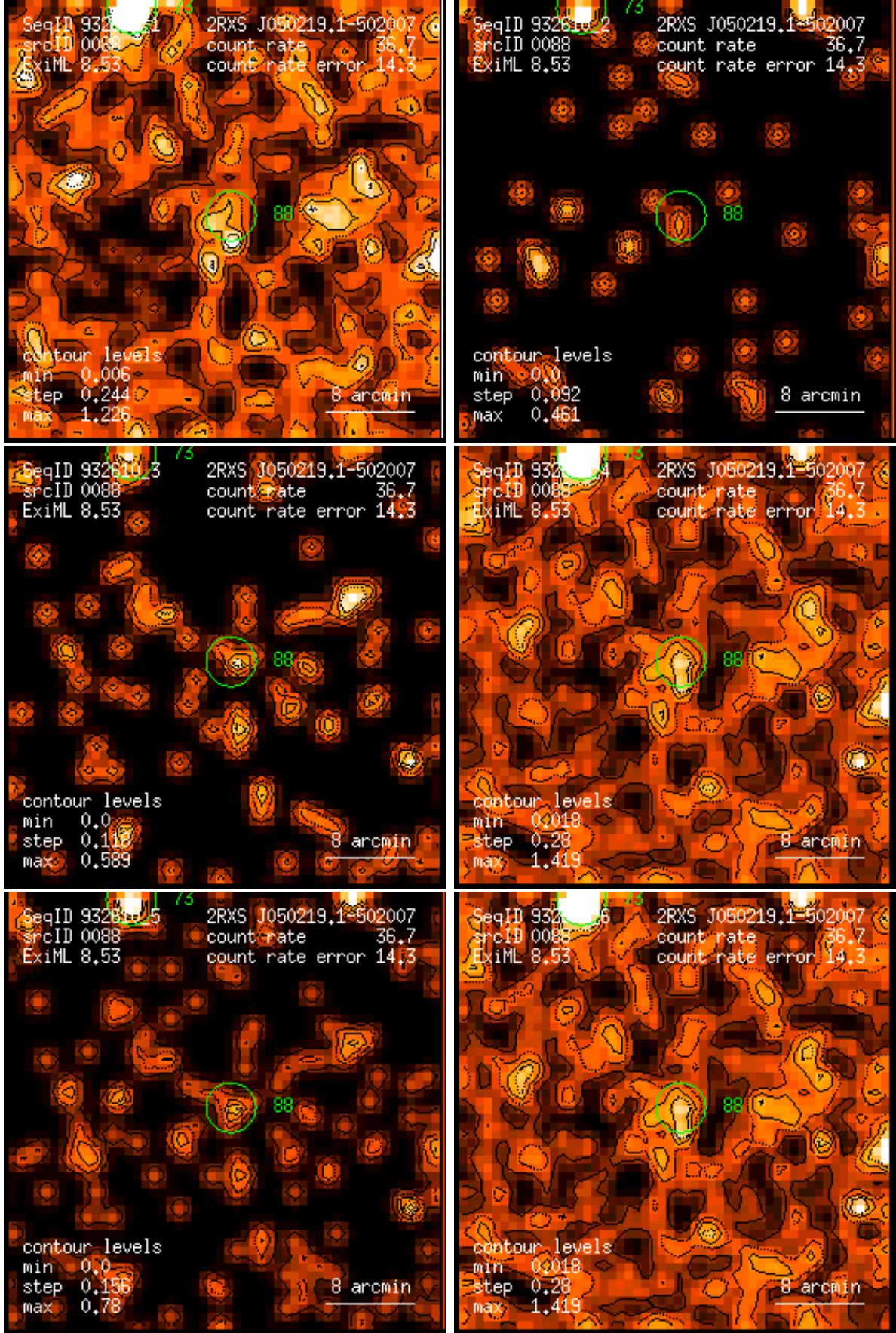
Figure 88: RASS 932610: detection 0088: band rate images, Gaussian filter: (1) PSPC channels 11 – 41, (2) 52 – 90, (3) 91 – 201, (4) 11 – 235, (5) 52 – 201, (6) 11 – 201. Broad band rates in counts/ks. Band rate contour levels in counts/ks/arcmin 2 .
