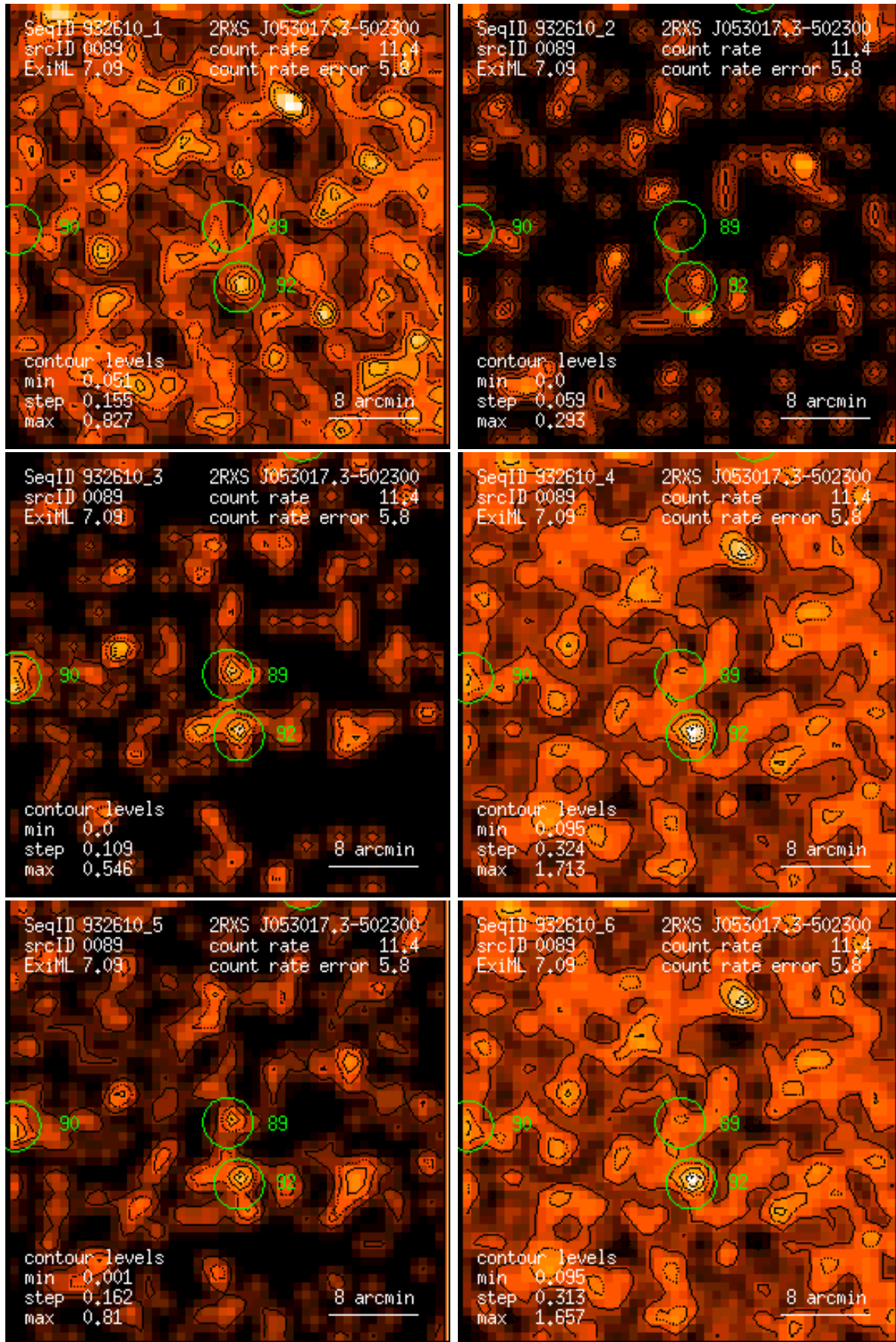
Figure 89: RASS 932610: detection 0089: band rate images, Gaussian filter: (1) PSPC channels 11 – 41, (2) 52 – 90, (3) 91 – 201, (4) 11 – 235, (5) 52 – 201, (6) 11 – 201. Broad band rates in counts/ks. Band rate contour levels in counts/ks/arcmin 2 .
