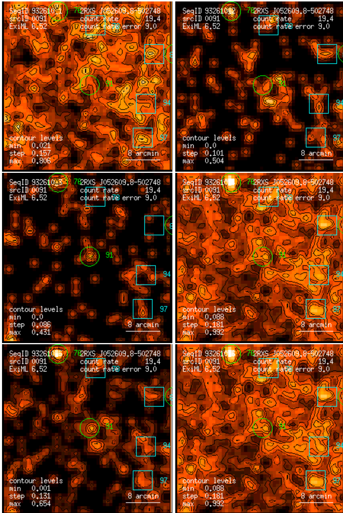
Figure 91: RASS 932610: detection 0091: band rate images, Gaussian filter: (1) PSPC channels 11 – 41, (2) 52 – 90, (3) 91 – 201, (4) 11 – 235, (5) 52 – 201, (6) 11 – 201. Broad band rates in counts/ks. Band rate contour levels in counts/ks/arcmin 2 .
