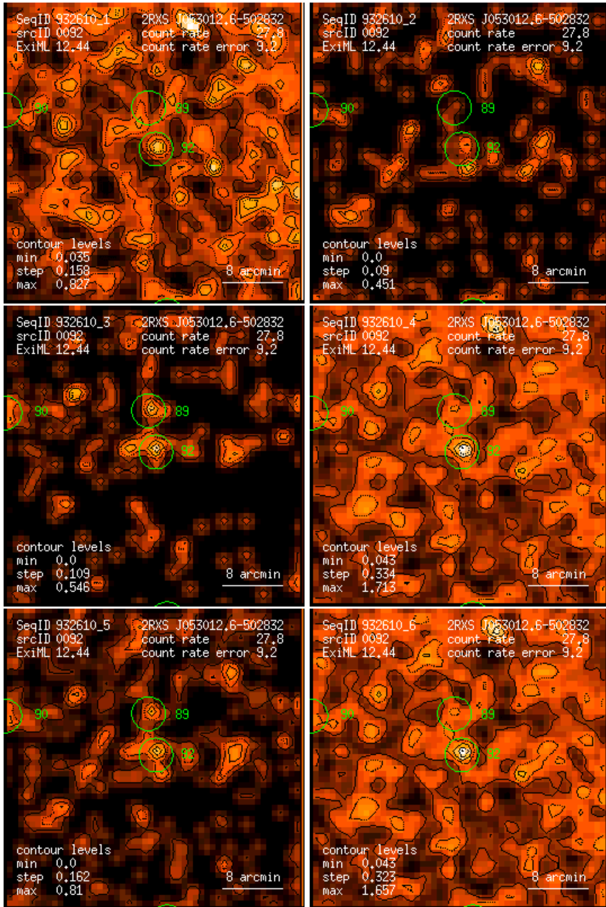
Figure 92: RASS 932610: detection 0092: band rate images, Gaussian filter: (1) PSPC channels 11 – 41, (2) 52 – 90, (3) 91 – 201, (4) 11 – 235, (5) 52 – 201, (6) 11 – 201. Broad band rates in counts/ks. Band rate contour levels in counts/ks/arcmin 2 .
