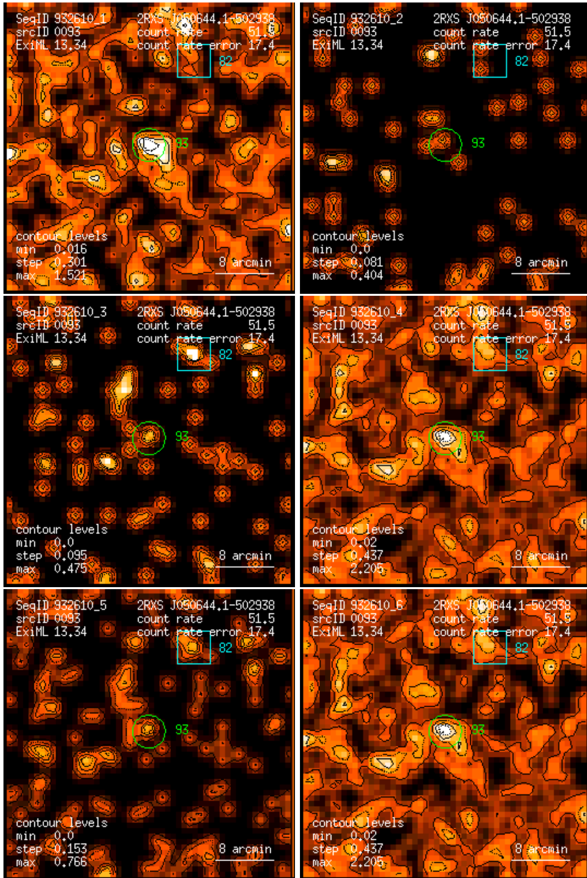
Figure 93: RASS 932610: detection 0093: band rate images, Gaussian filter: (1) PSPC channels 11 – 41, (2) 52 – 90, (3) 91 – 201, (4) 11 – 235, (5) 52 – 201, (6) 11 – 201. Broad band rates in counts/ks. Band rate contour levels in counts/ks/arcmin 2 .
