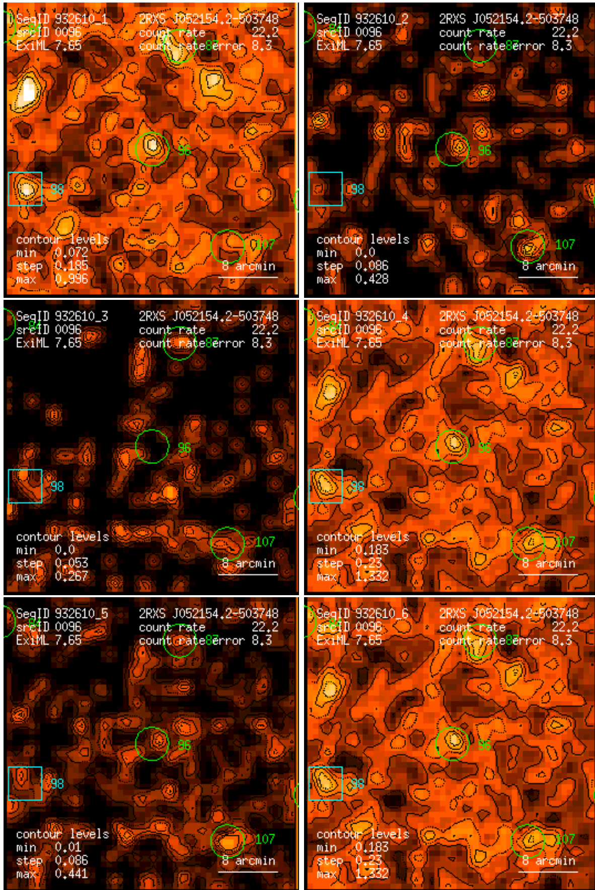
Figure 96: RASS 932610: detection 0096: band rate images, Gaussian filter: (1) PSPC channels 11 – 41, (2) 52 – 90, (3) 91 – 201, (4) 11 – 235, (5) 52 – 201, (6) 11 – 201. Broad band rates in counts/ks. Band rate contour levels in counts/ks/arcmin 2 .
