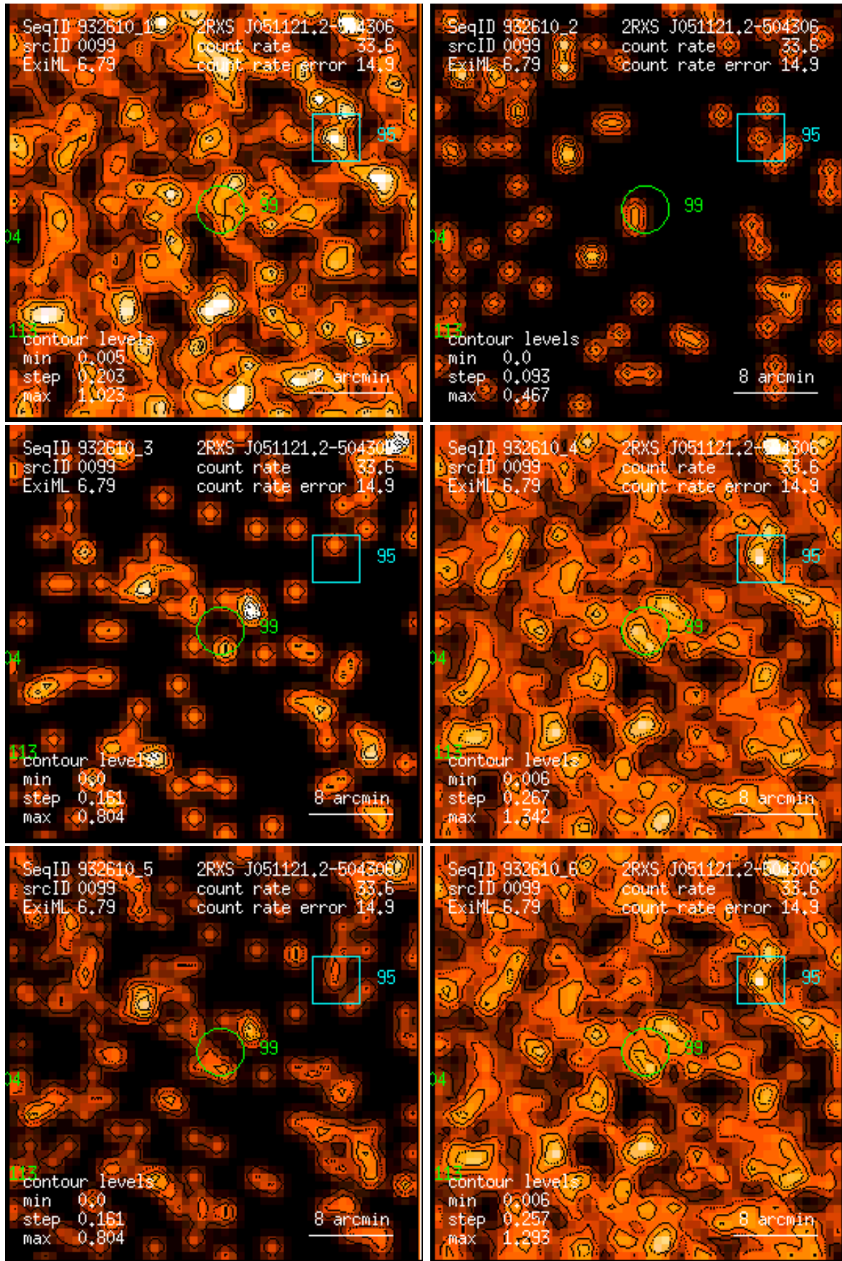
Figure 99: RASS 932610: detection 0099: band rate images, Gaussian filter: (1) PSPC channels 11 – 41, (2) 52 – 90, (3) 91 – 201, (4) 11 – 235, (5) 52 – 201, (6) 11 – 201. Broad band rates in counts/ks. Band rate contour levels in counts/ks/arcmin 2 .
