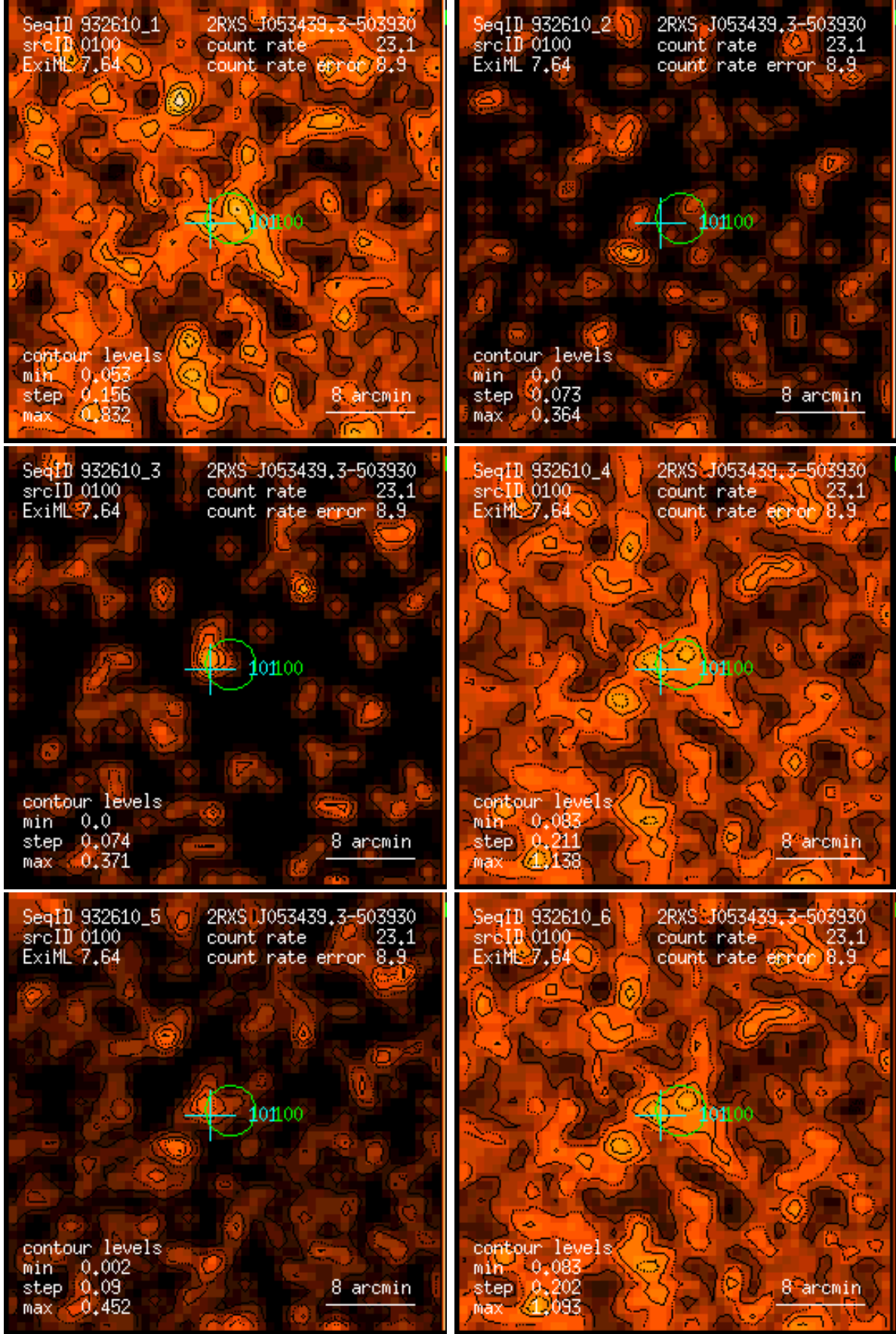
Figure 100: RASS 932610: detection 0100: band rate images, Gaussian filter: (1) PSPC channels 11 – 41, (2) 52 – 90, (3) 91 – 201, (4) 11 – 235, (5) 52 – 201, (6) 11 – 201. Broad band rates in counts/ks. Band rate contour levels in counts/ks/arcmin 2 .
