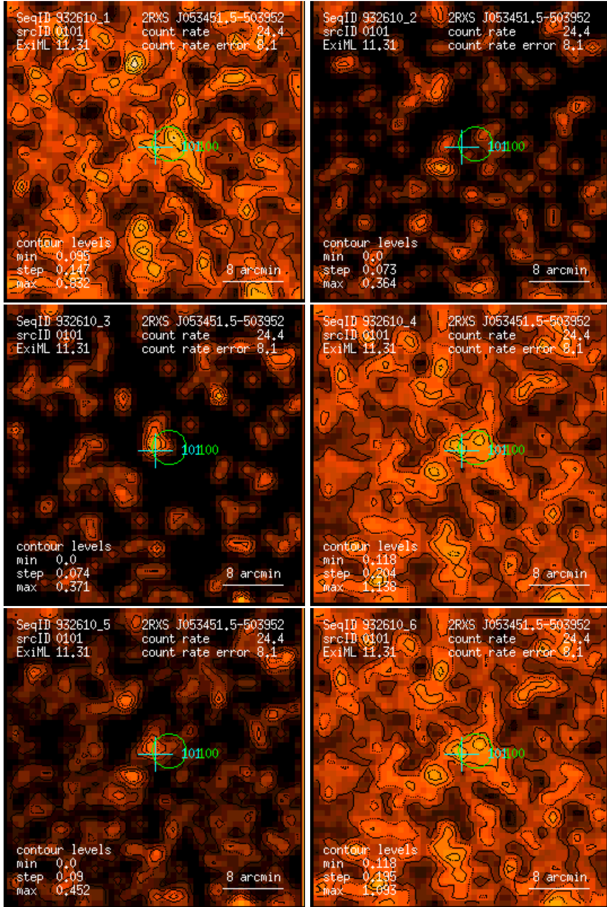
Figure 101: RASS 932610: detection 0101: band rate images, Gaussian filter: (1) PSPC channels 11 – 41, (2) 52 – 90, (3) 91 – 201, (4) 11 – 235, (5) 52 – 201, (6) 11 – 201. Broad band rates in counts/ks. Band rate contour levels in counts/ks/arcmin 2 .
