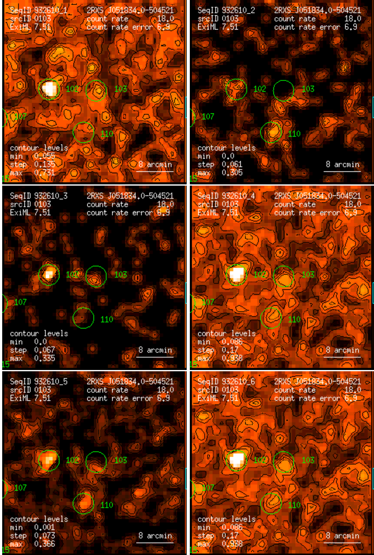
Figure 103: RASS 932610: detection 0103: band rate images, Gaussian filter: (1) PSPC channels 11 – 41, (2) 52 – 90, (3) 91 – 201, (4) 11 – 235, (5) 52 – 201, (6) 11 – 201. Broad band rates in counts/ks. Band rate contour levels in counts/ks/arcmin 2 .
