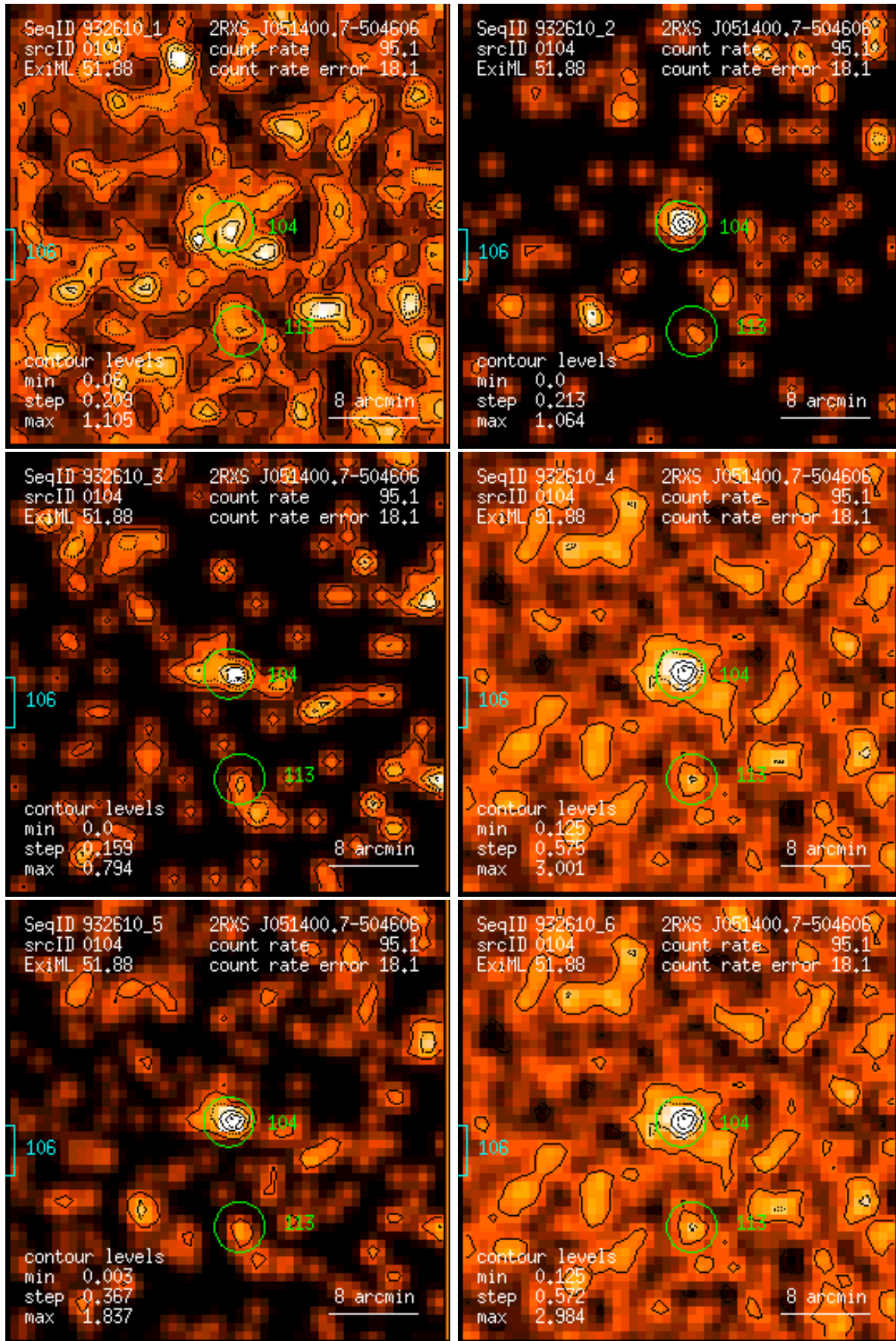
Figure 104: RASS 932610: detection 0104: band rate images, Gaussian filter: (1) PSPC channels 11 – 41, (2) 52 – 90, (3) 91 – 201, (4) 11 – 235, (5) 52 – 201, (6) 11 – 201. Broad band rates in counts/ks. Band rate contour levels in counts/ks/arcmin 2 .
